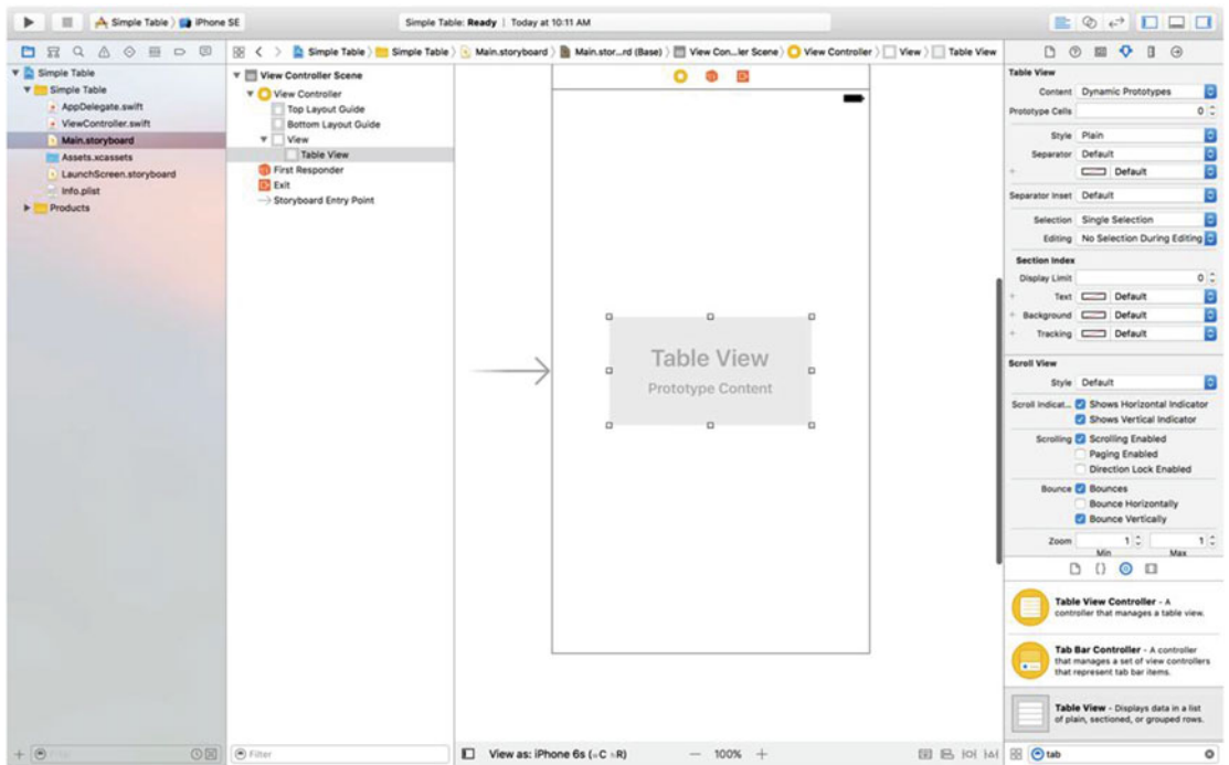
Figure 8-4. Dragging a table view from the library onto our main view
