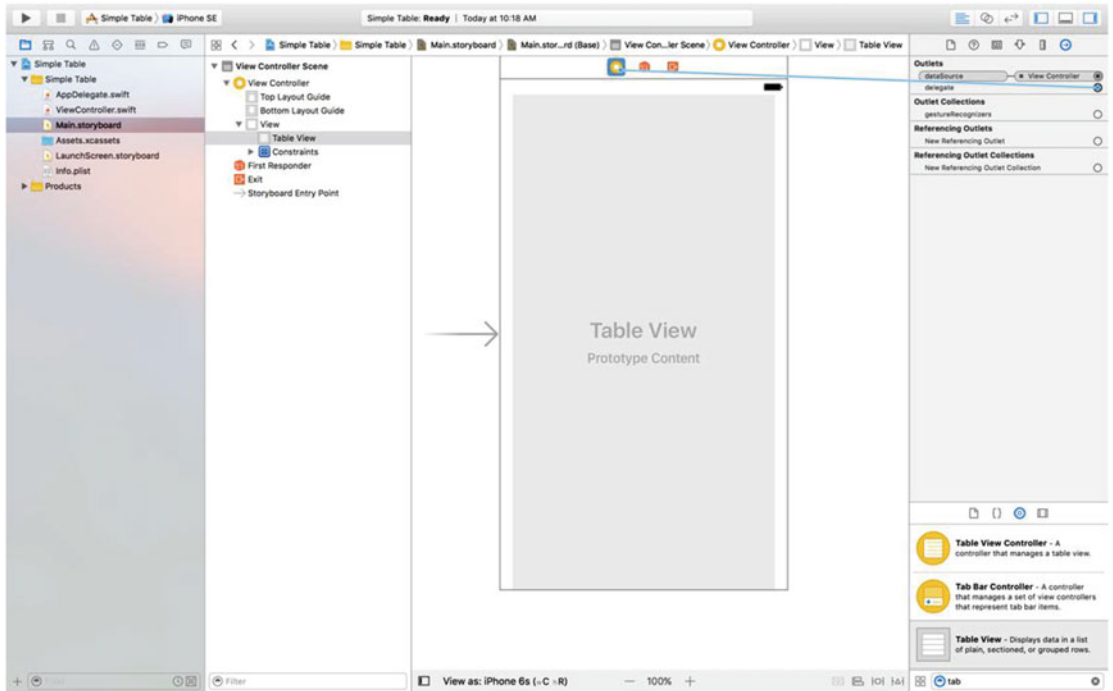
Figure 8-6. Connecting our Table View's dataSource and delegate outlets
