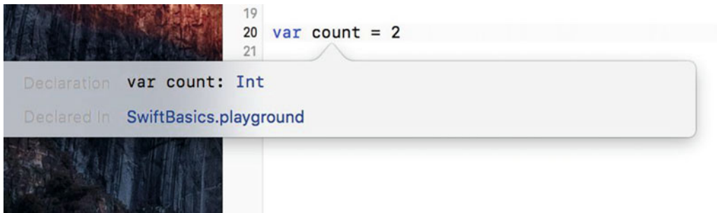
Figure A-2. Getting the inferred type of a variable
