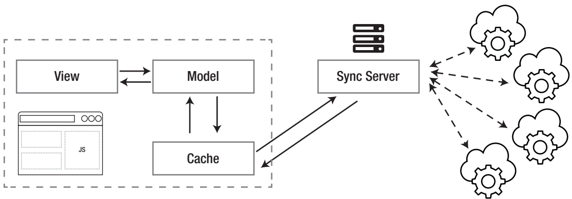
Figure 9-3. Offline first approach with syncing in mind
