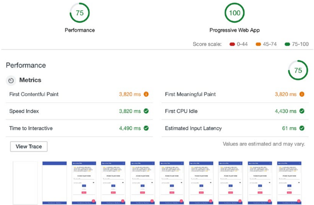
Figure 7-9. Audit website in Chrome audit tab to check performance score before deploying App Shell implementation on simulated mobile fast 3G
