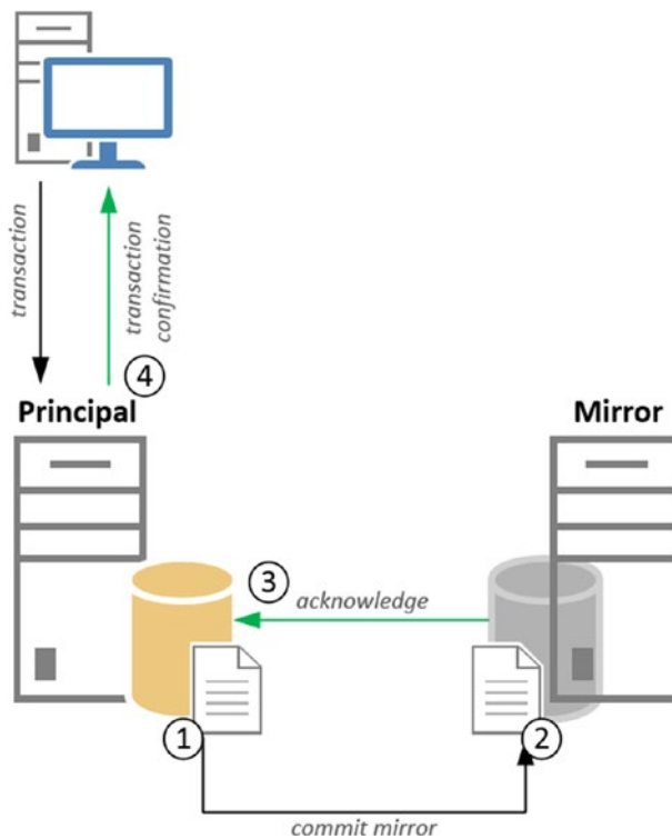
Figure 10-1. Synchronous mirroring
