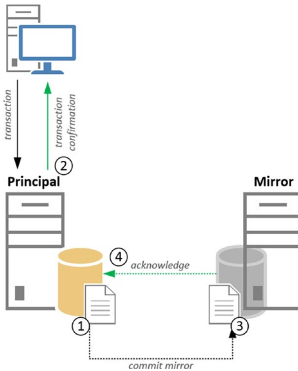
Figure 10-2. Asynchronous mirroring
