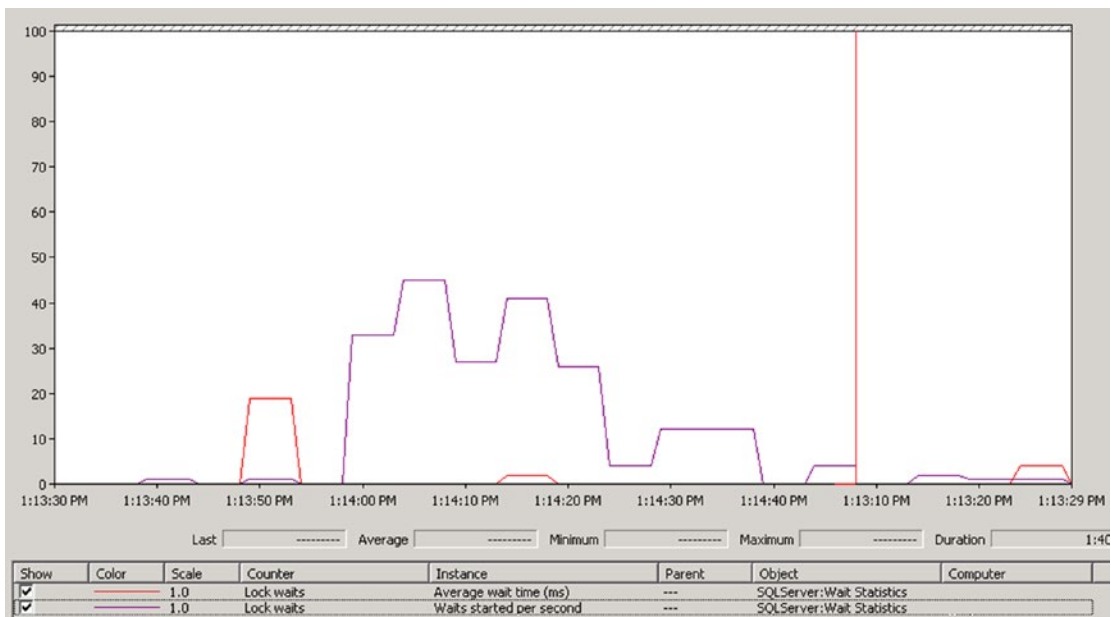
Figure 2-16. Perfmon graph showing wait statistics information
