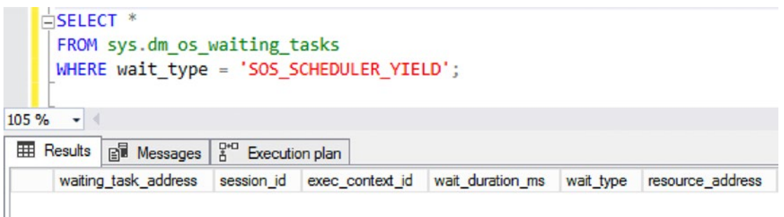
Figure 5-14. No SOS_SCHEDULER_YIELD waits occurring
