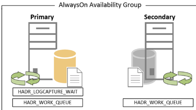
Figure 10-7. HADR_LOGCAPTURE_WAIT and HADR_WORK_QUEUE wait types
