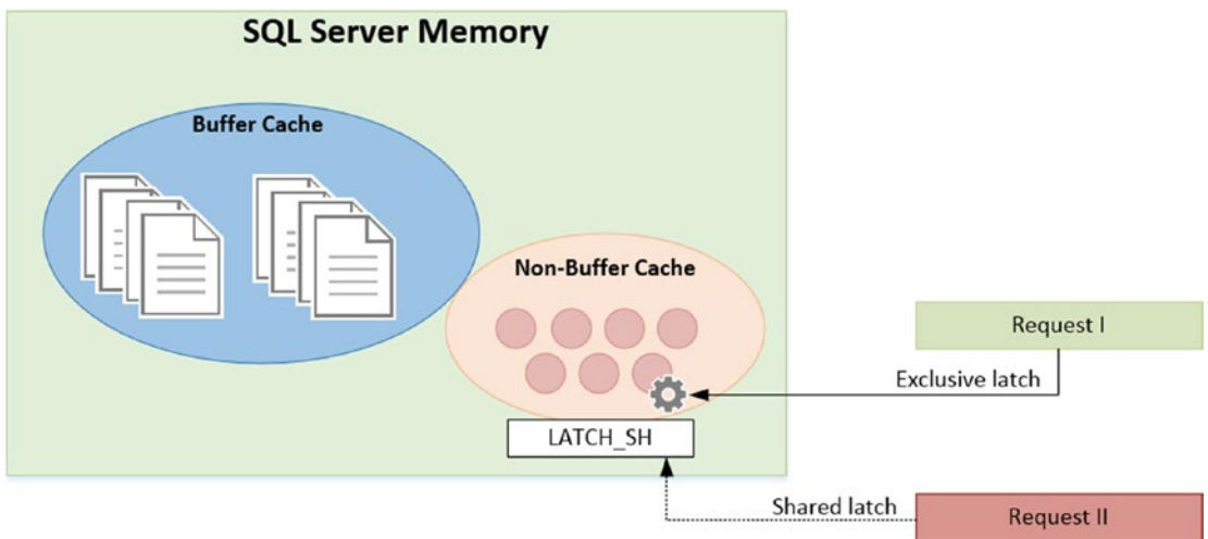
Figure 9-17. LATCH_SH wait occurring
