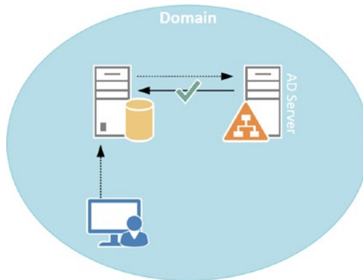
Figure 11-15. SQL Server Windows login authentication inside domain
