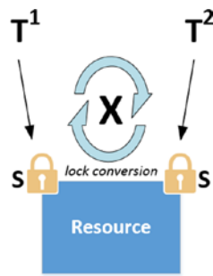
Figure 8-14. Deadlock during lock conversion
