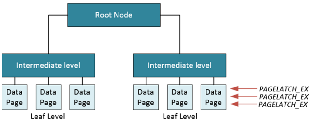
Figure 9-9. Last-page insert contention on last page in a clustered index
