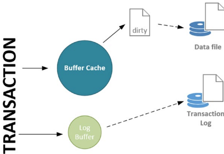
Figure 6-16. How a transaction moves
