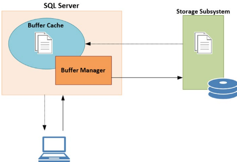
Figure 9-23. Moving a page from the storage subsystem to the buffer cache
