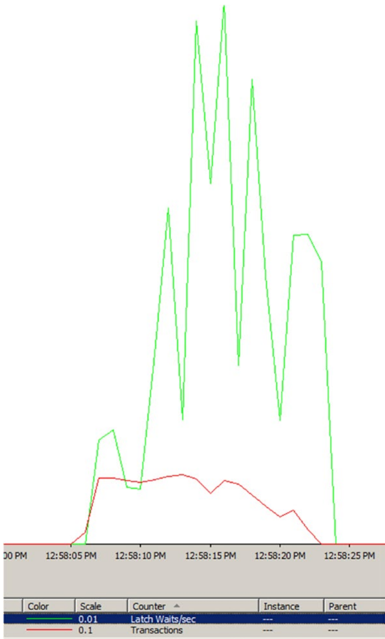
Figure 9-6. Latch Waits/sec and Transactions Perfmon graph
