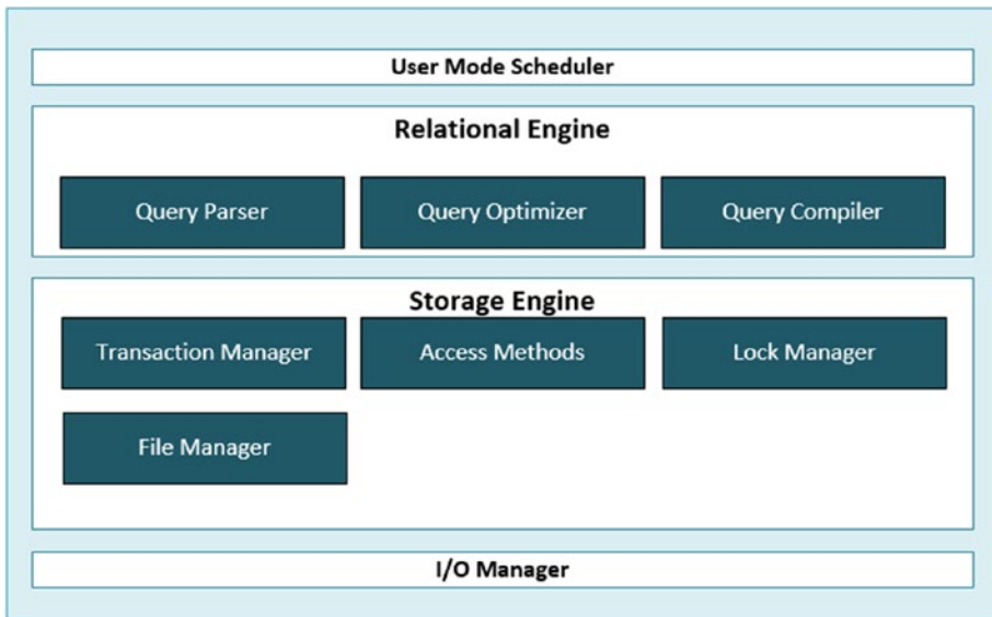
Figure 1-3. SQL Server architecture before the introduction of the SQLOS
