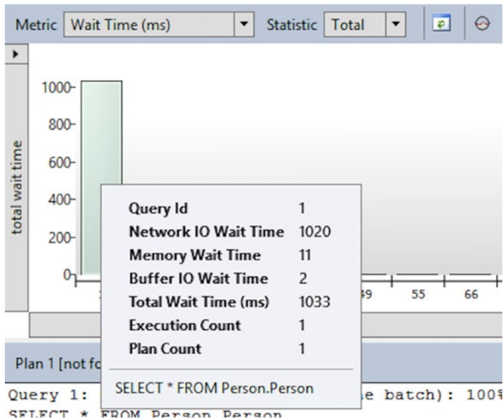
Figure 3-4. Wait categories exposed in the Query Store
