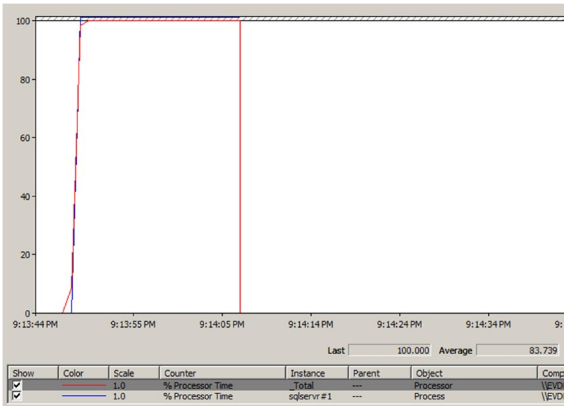
Figure 5-13. Impact of Ostress on the CPU
