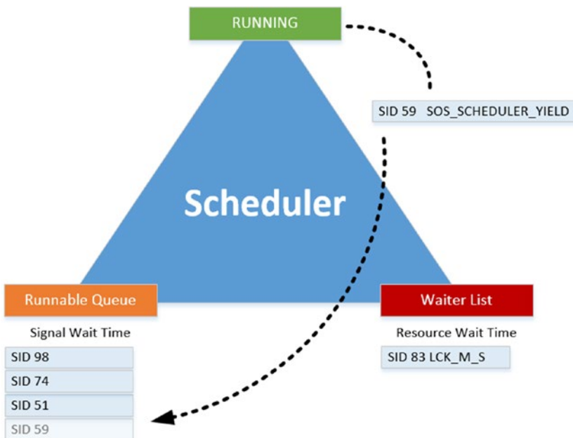
Figure 5-10. Worker thread voluntarily yielding the processor
