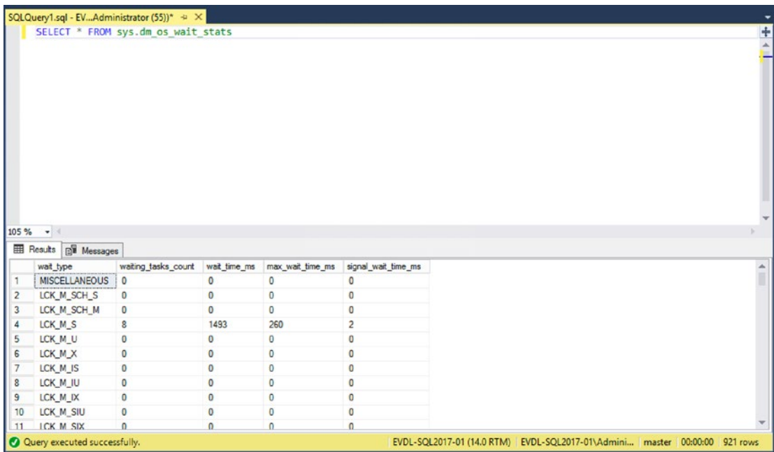
Figure 1-2. SQL Server wait statistics in SQL Server 2017
