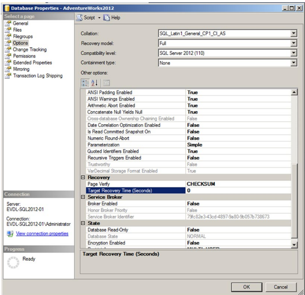
Figure 12-4. Indirect checkpoint feature location and value
