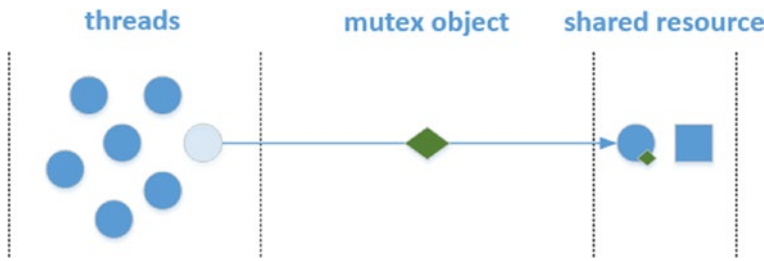
Figure 6-12. Thread waiting for a Mutex object to access a shared resource
