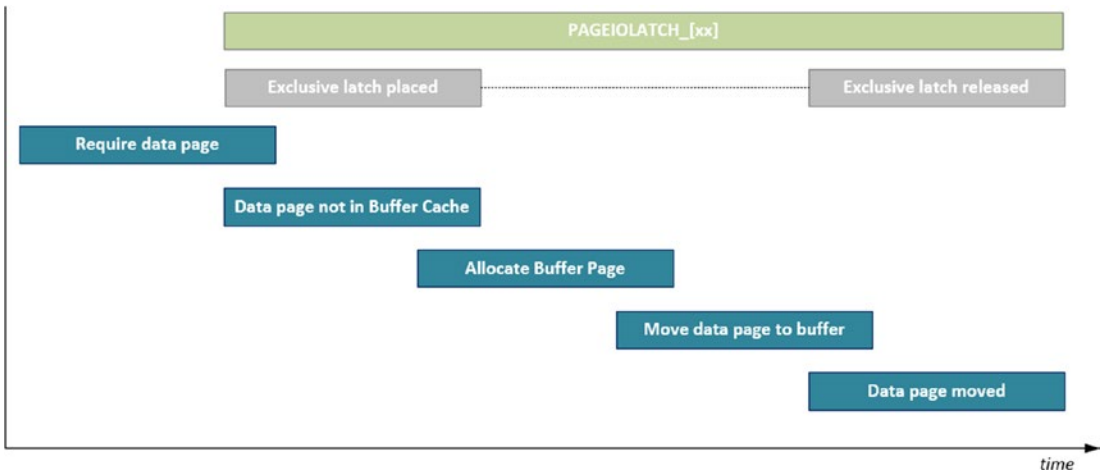
Figure 9-24. Movement of data page
