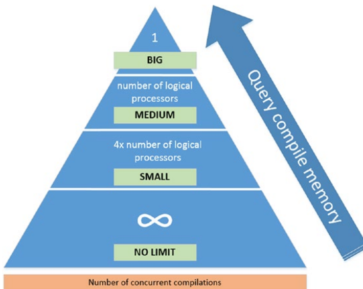
Figure 6-24. Compilation-memory resource semaphore
