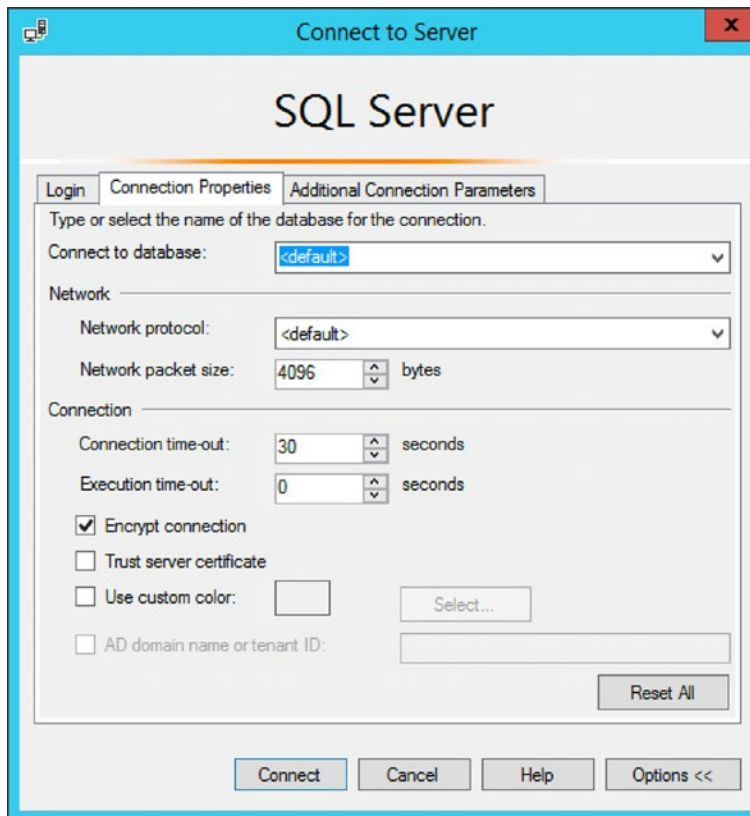
Figure 11-10. Connection Properties in SQL Server Management Studio
