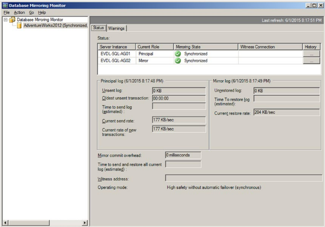
Figure 10-5. Database mirroring monitor
