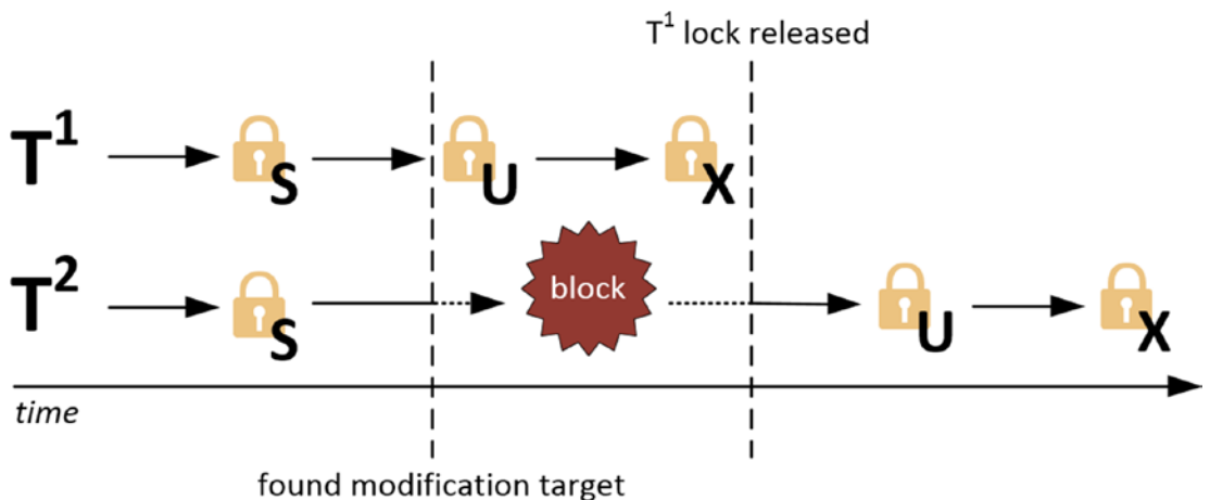
Figure 8-15. Update locks during concurrent data modifications
