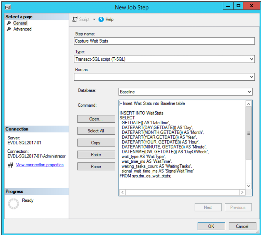
Figure 4-7. Capturing WaitStats SQL Server Agent job step
