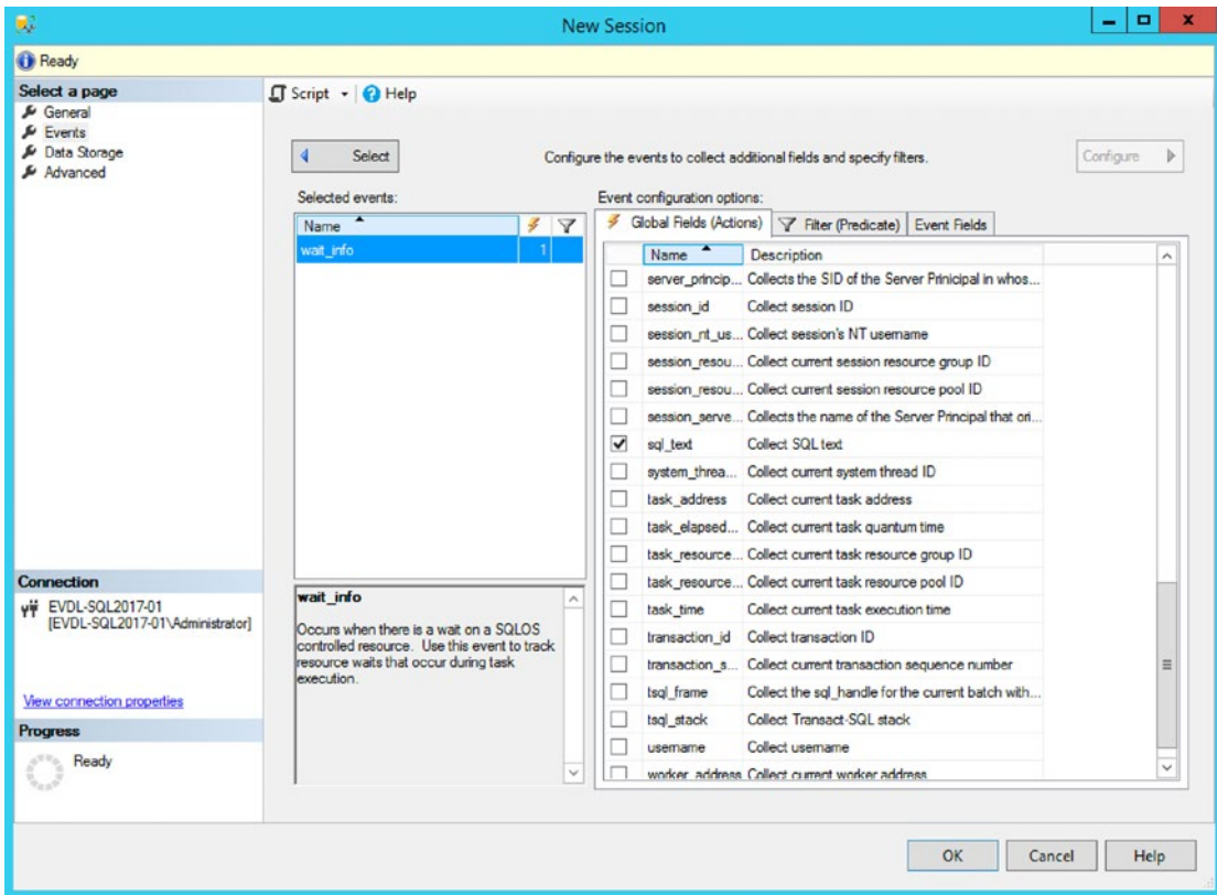
Figure 2-21. Setting the sql_text global field
