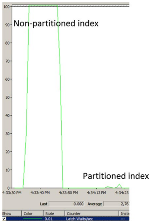
Figure 9-15. Latch Waits/sec against both a non-partitioned and a partitioned index
