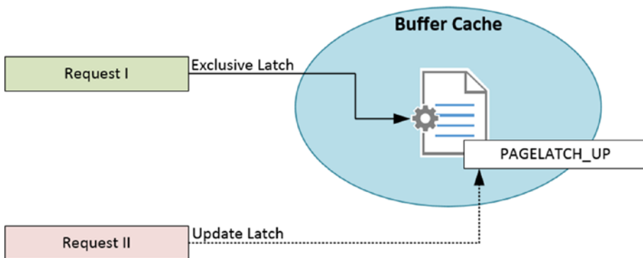
Figure 9-8. PAGELATCH_UP wait occurring
