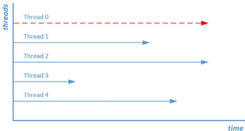
Figure 5-7. Skewed parallel query threading
