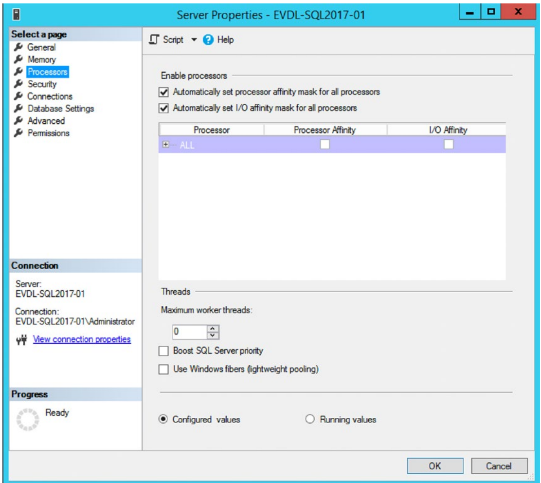
Figure 5-18. Processors configuration of a SQL Server instance
