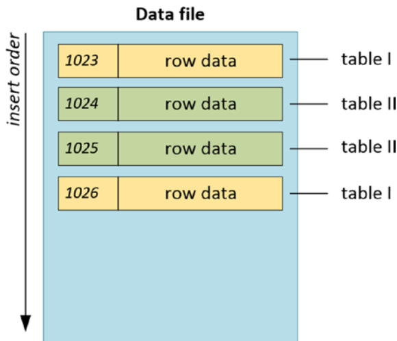
Figure 13-1. Memory-optimized table's data file
