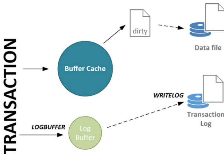
Figure 6-17. Transaction movement and the LOGBUFFER and WRITELOG wait types
