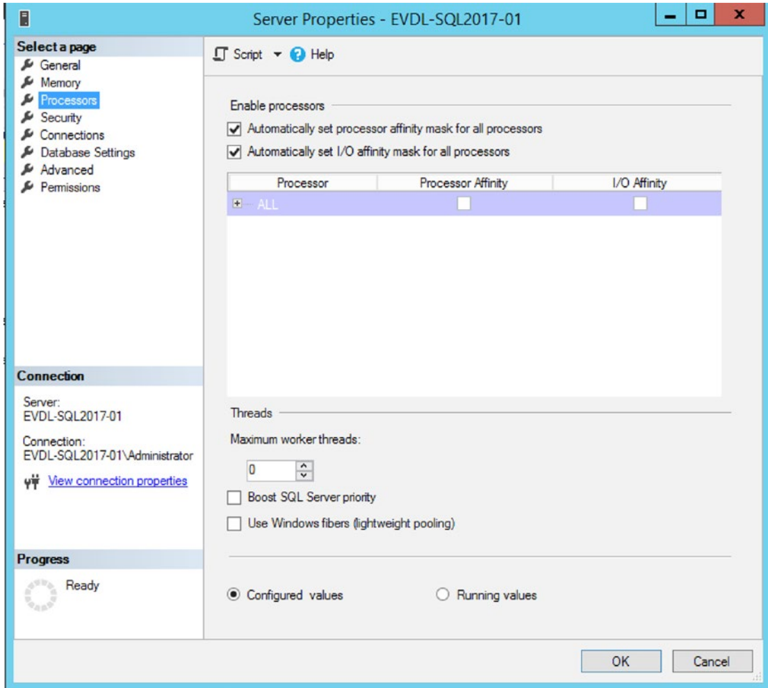
Figure 1-9. Processors page in the Server Properties
