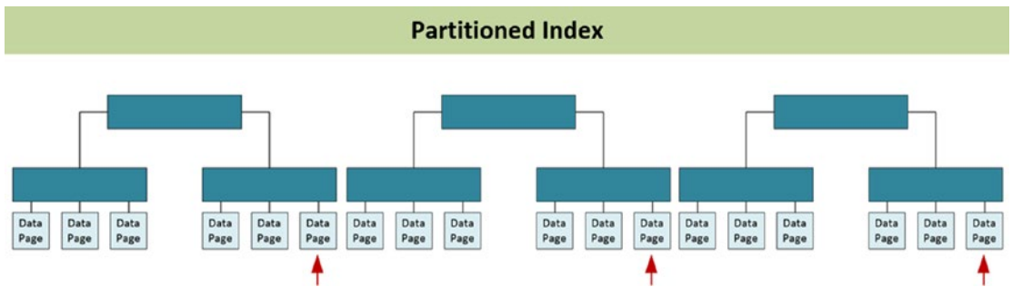
Figure 9-14. Last-page inserts spread across partitions
