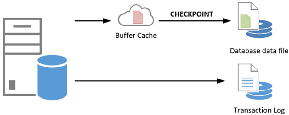
Figure 6-29. Data modification process
