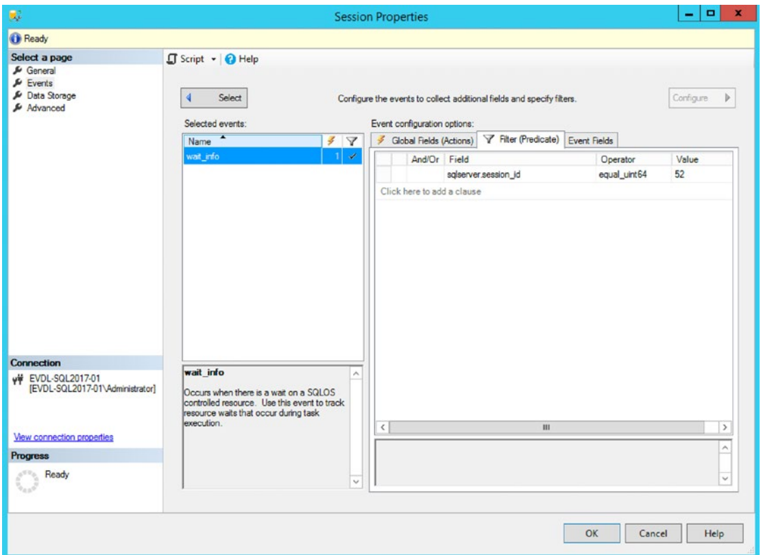
Figure 2-22. Setting an event filter
