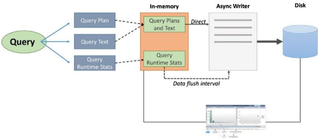
Figure 3-1. Query Store architecture
