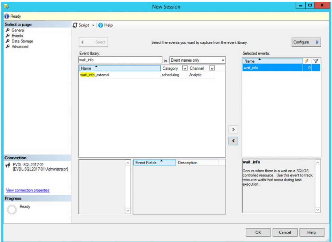
Figure 2-20. Selecting an event to monitor
