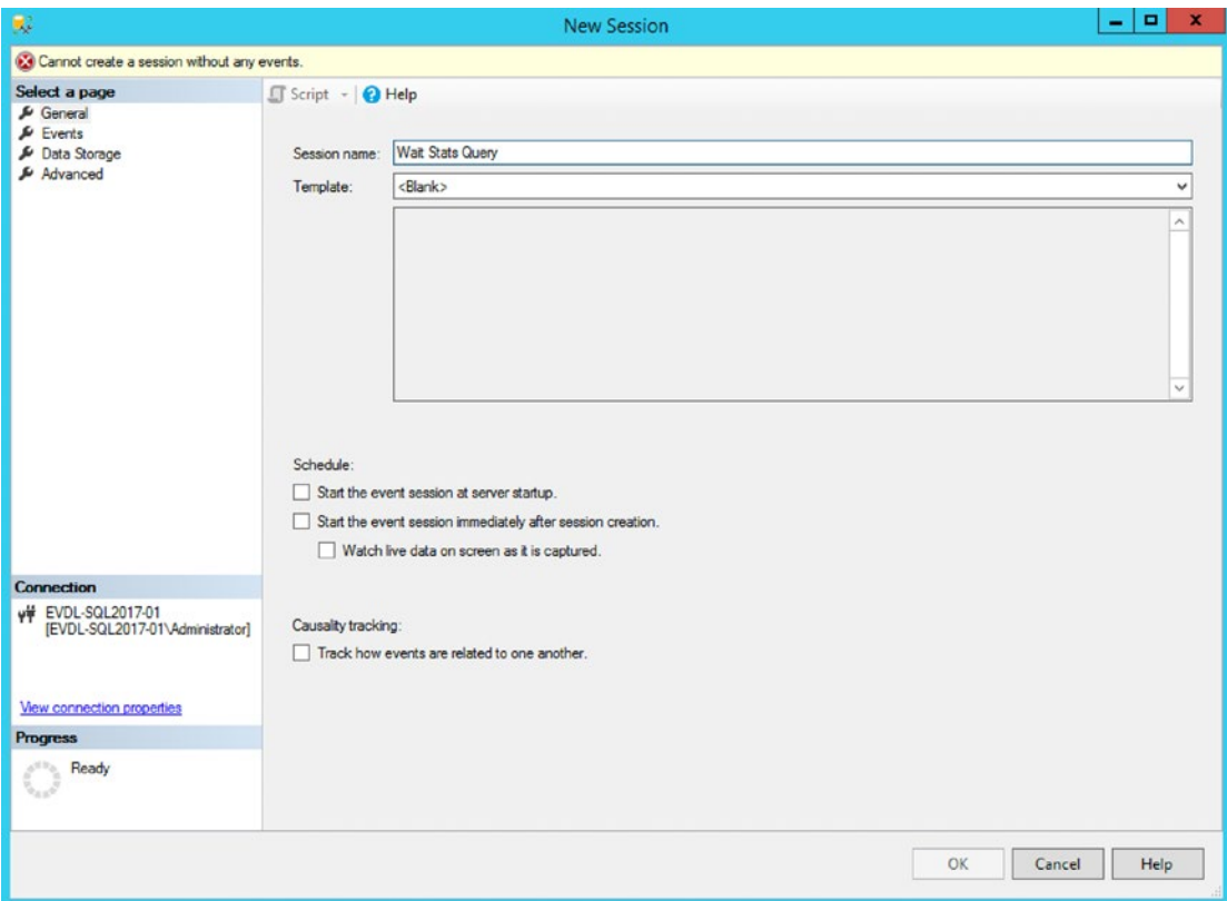
Figure 2-19. Configuring wait statistics Extended Event session
