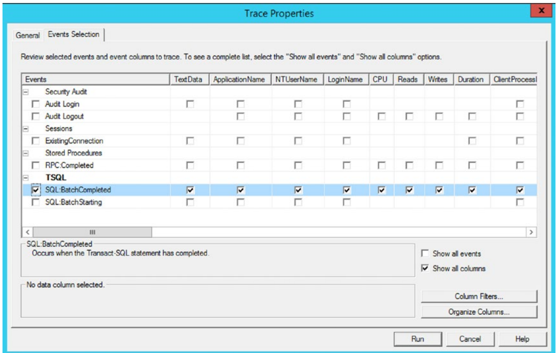
Figure 12-12. SQL:BatchCompleted event selected
