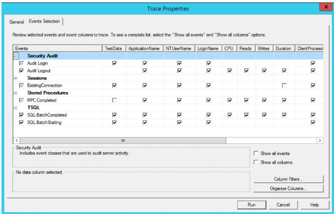
Figure 12-11. SQL Server Profiler default event selection
