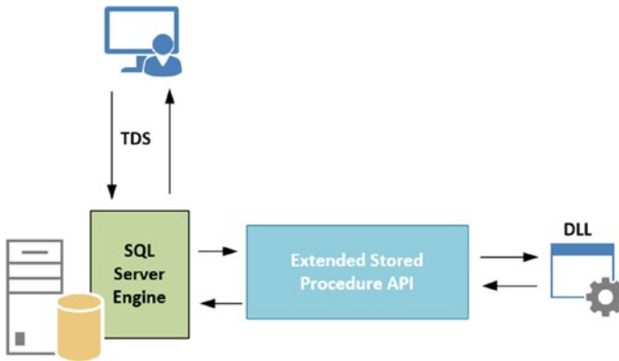
Figure 11-18. Executing an extended stored procedure
