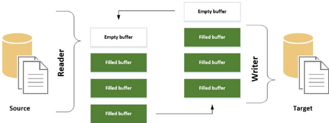
Figure 7-5. Internals of a backup operation
