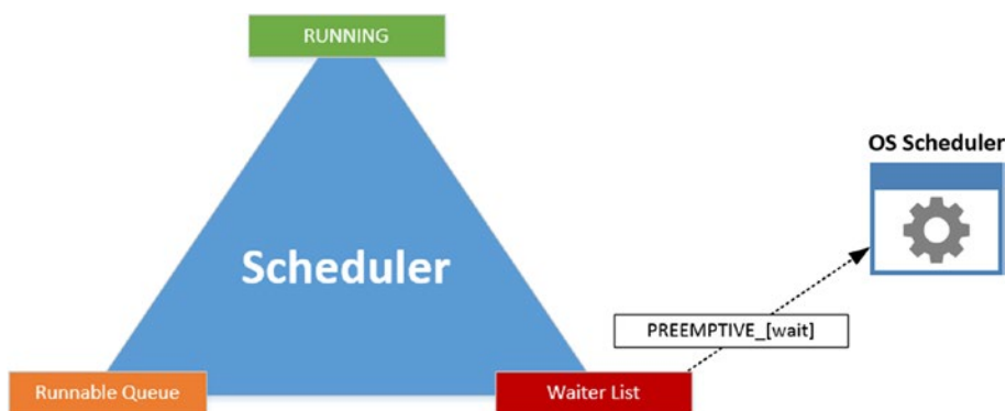
Figure 11-1. Preemptive wait occurring
