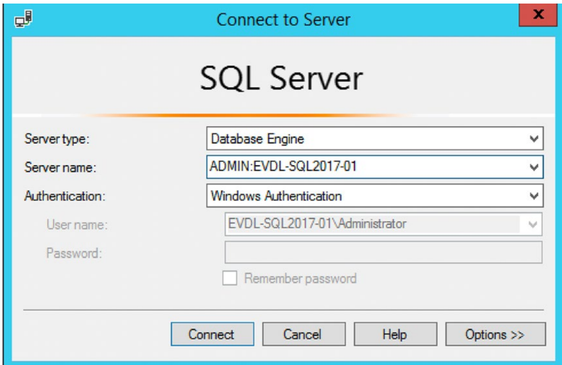
Figure 5-25. Connect using the Dedicated Administrator Connection
