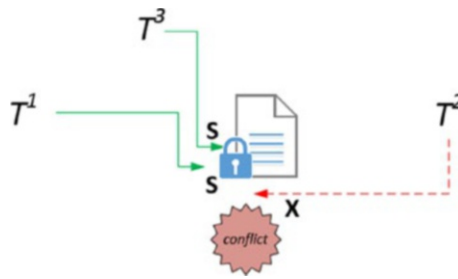
Figure 8-1. Concurrent lock situation
