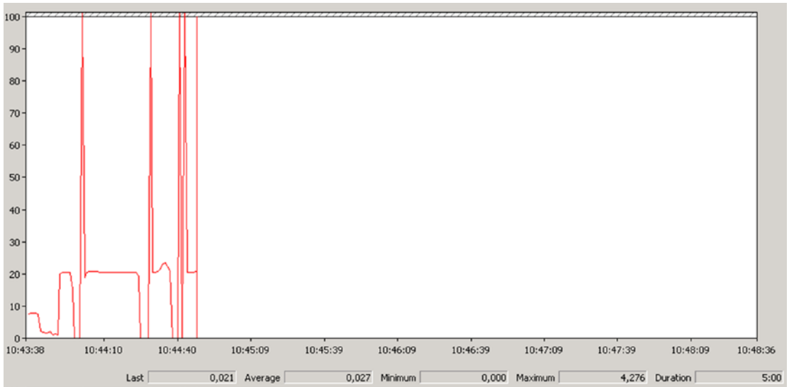
Figure 4-14. Disk-read latency
