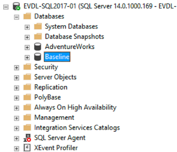
Figure 4-4. Baseline database
