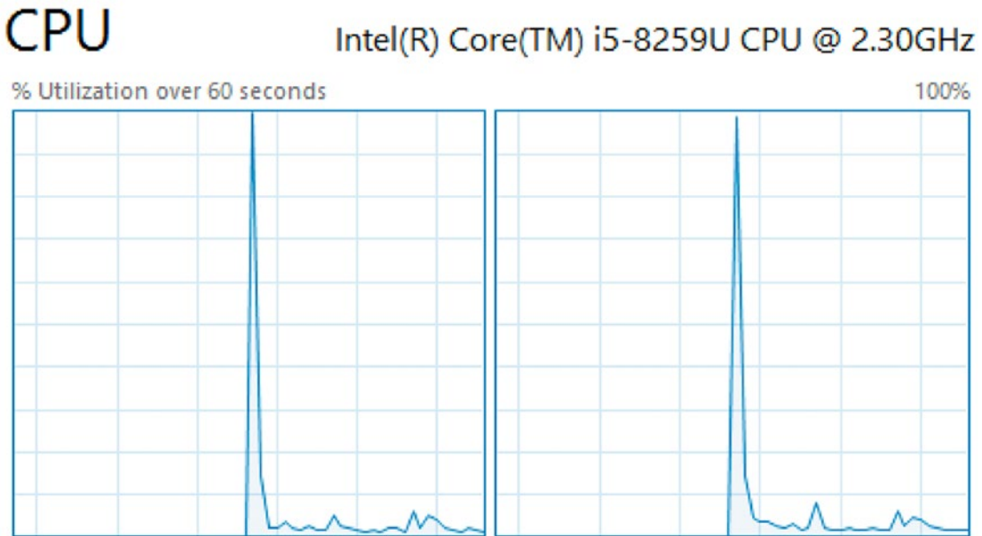
Figure 5-30. CPU usage
