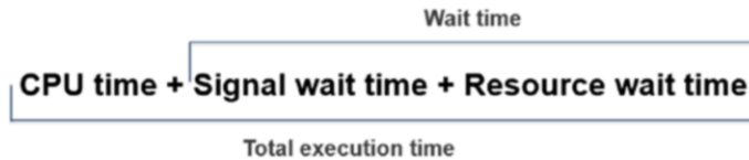
Figure 1-15. Request execution time calculation
