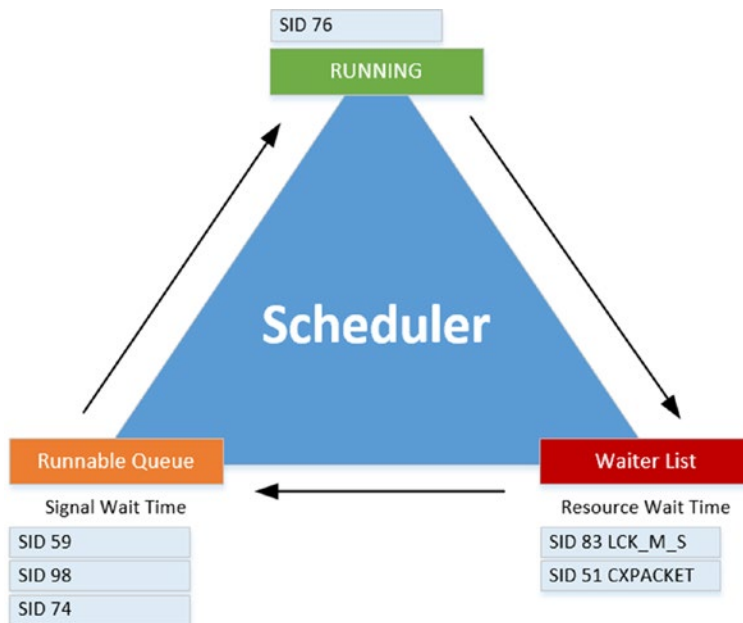
Figure 1-16. Scheduler with running requests
