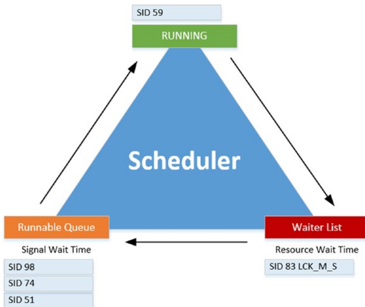
Figure 1-17. Scheduler a few milliseconds later
