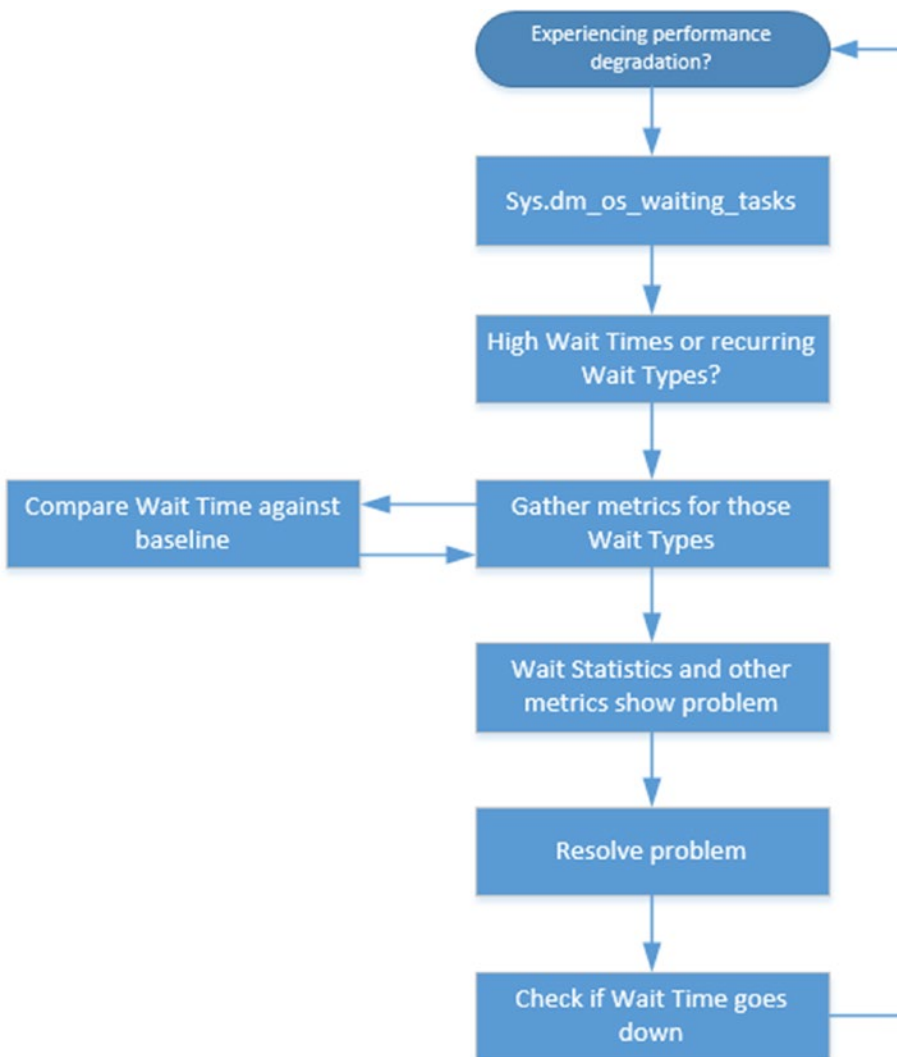
Figure 4-9. Complete wait statistics performance-analysis flowchart
