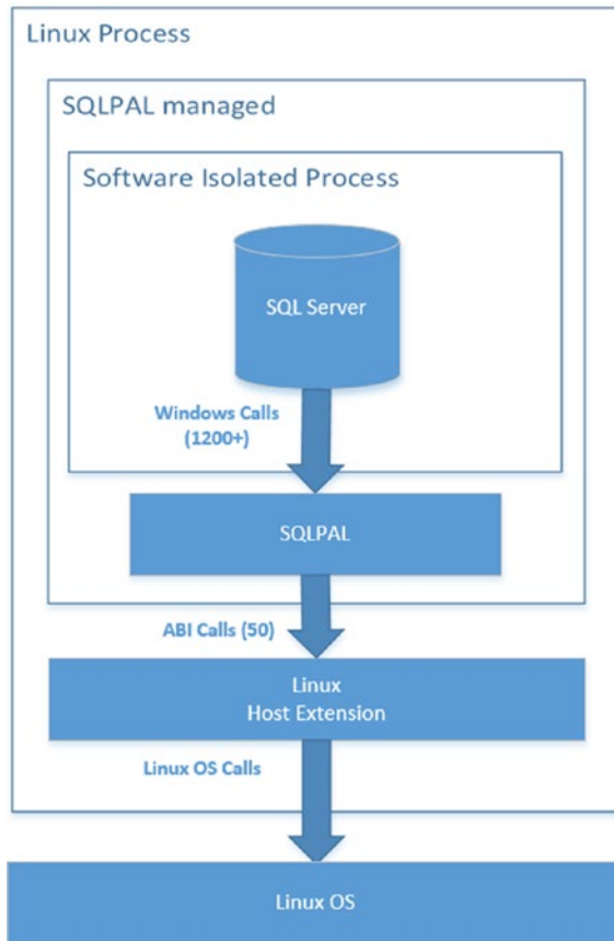
Figure 11-3. PAL layer interaction on SQL-on-Linux
