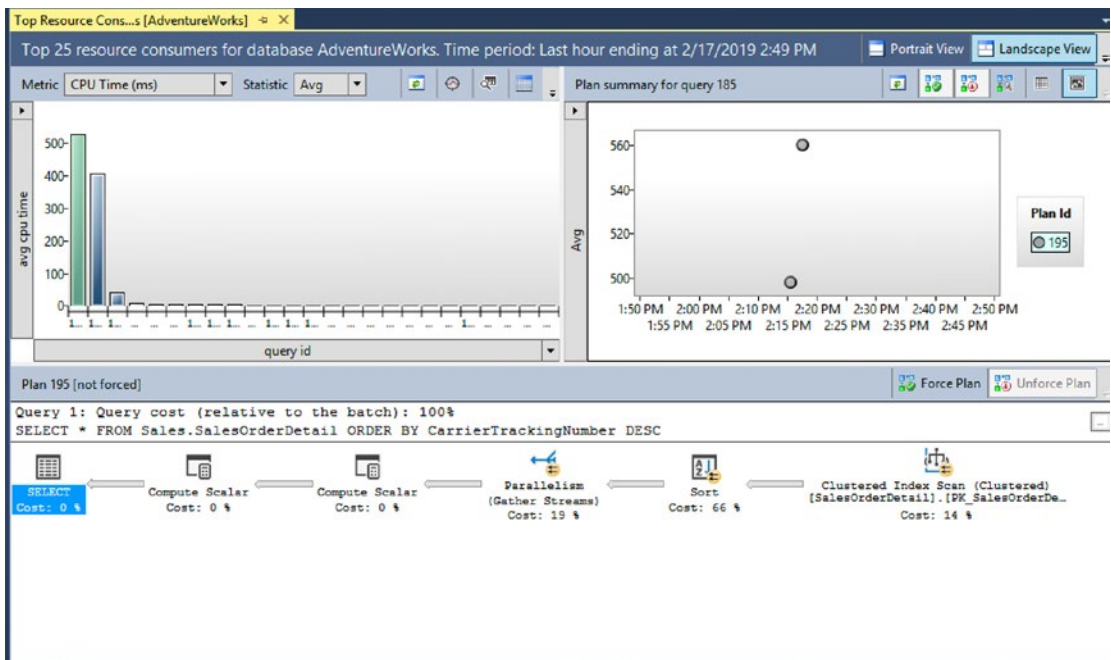
Figure 5-17. Visualizing expensive CPU queries through the Query Store
