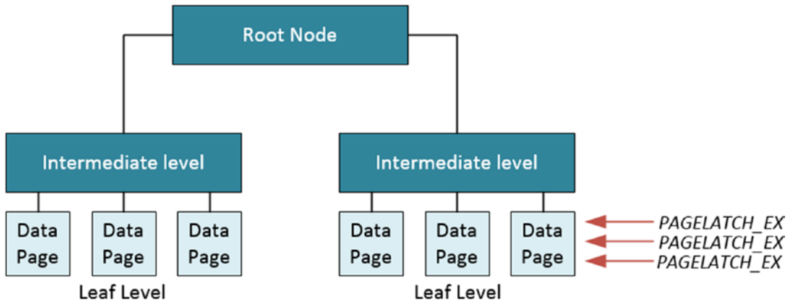
Figure 9-13. Last-page insert contention on the right-most data page of an index
