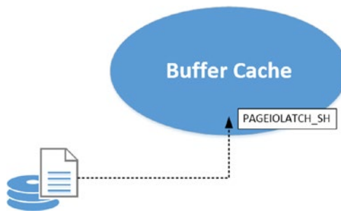
Figure 9-2. PAGEIOLATCH_SH occurring
