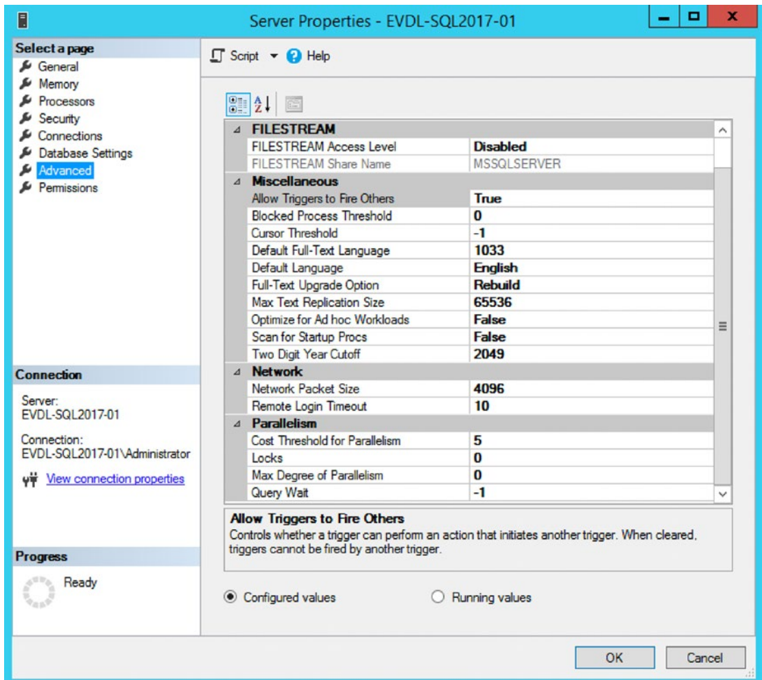
Figure 5-2. Parallelism configuration
