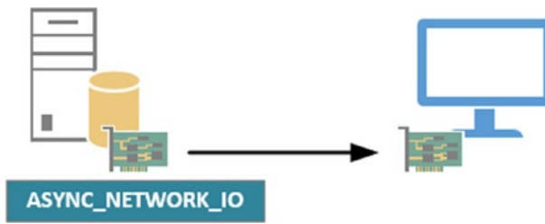
Figure 6-8. ASYNC_NETWORK_IO
