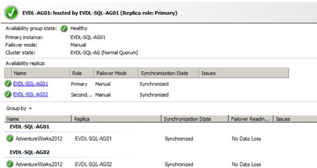
Figure 10-12. AlwaysOn Dashboard
