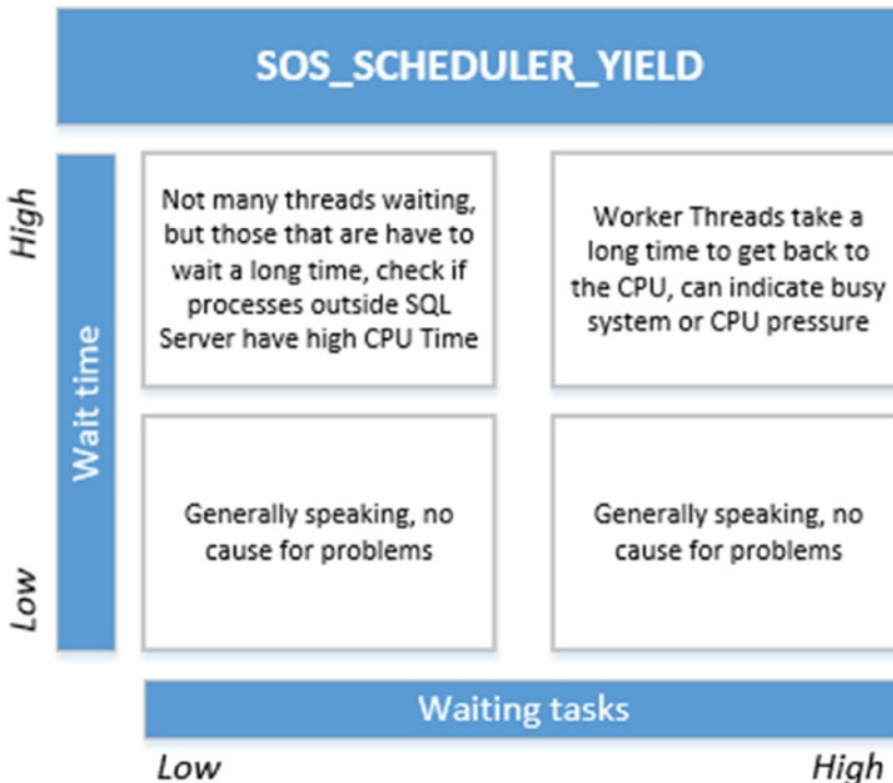
Figure 5-12. SOS_SCHEDULER_YIELD situations
