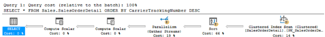
Figure 5-5. Actual execution plan without MAXDOP 1 option
