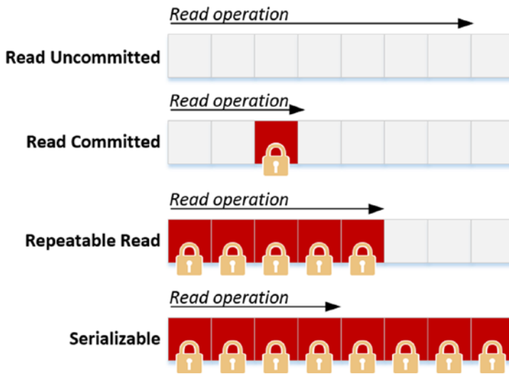
Figure 8-3. Isolation levels and locking behavior
