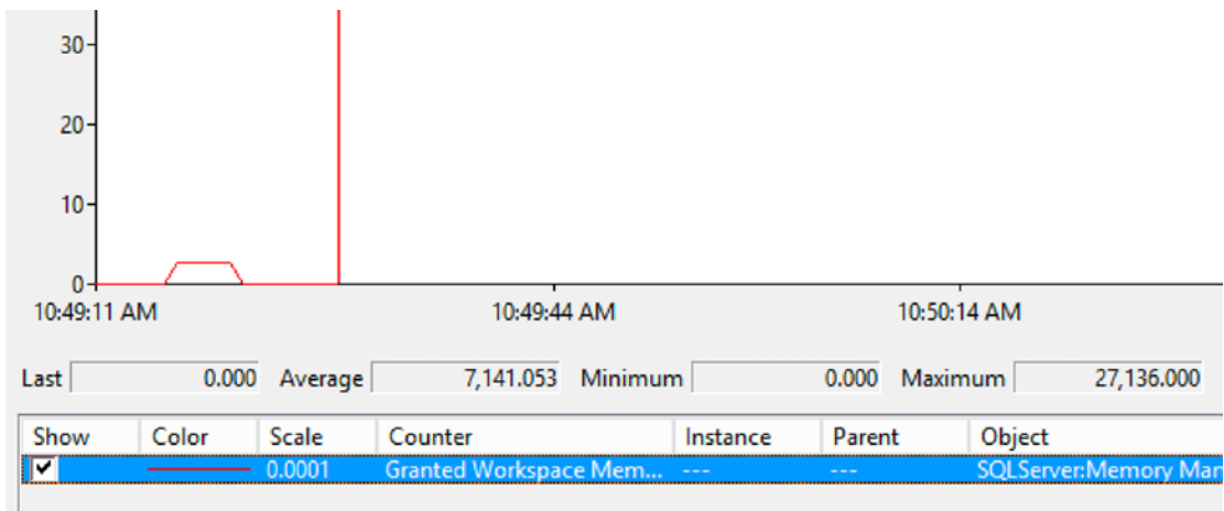
Figure 6-23. Granted Workspace Memory (KB) Perfmon counter
