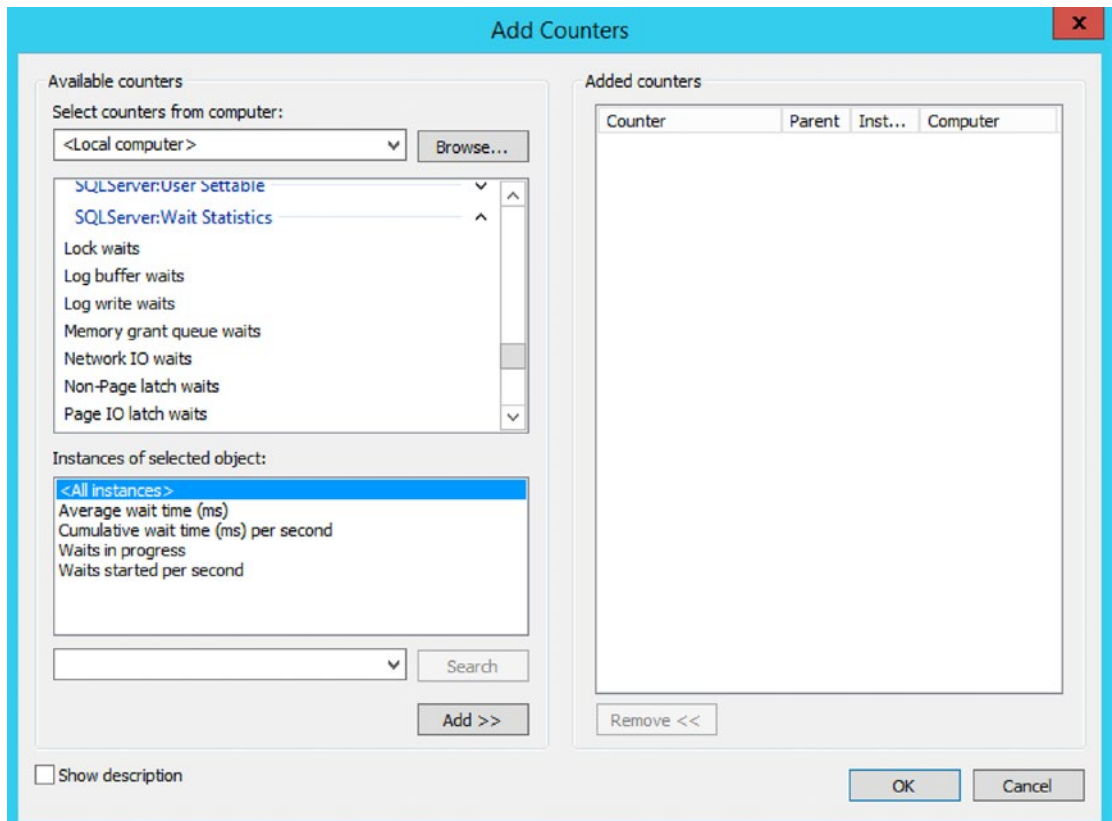
Figure 2-15. Wait statistics counters inside Perfmon
