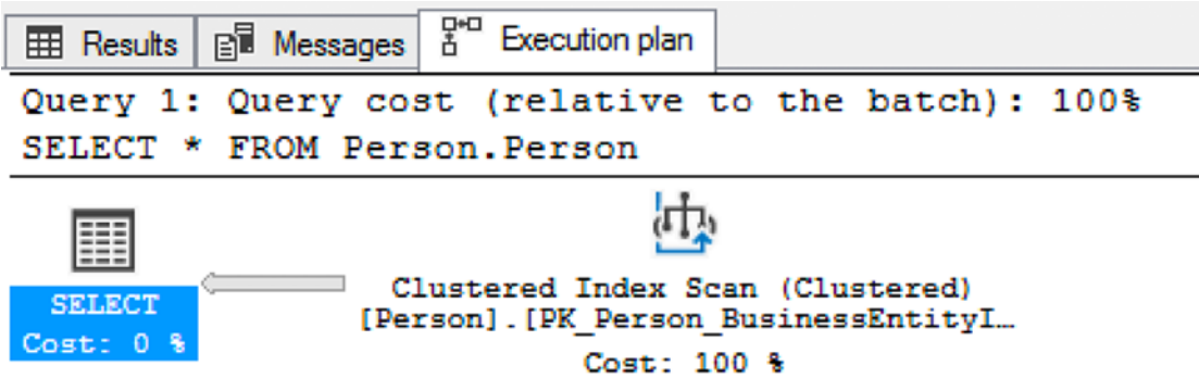
Figure 2-27. Execution plan
