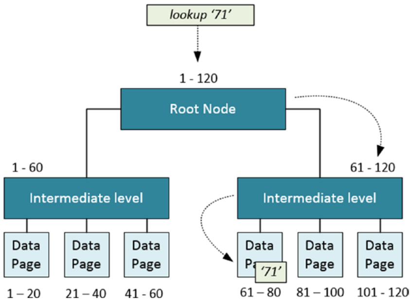
Figure 9-21. B-tree navigation
