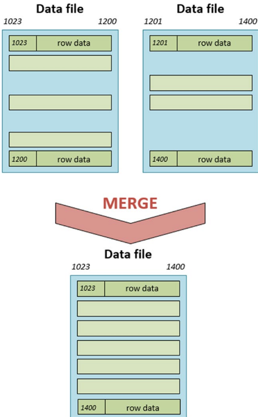
Figure 13-3. Merge operation
