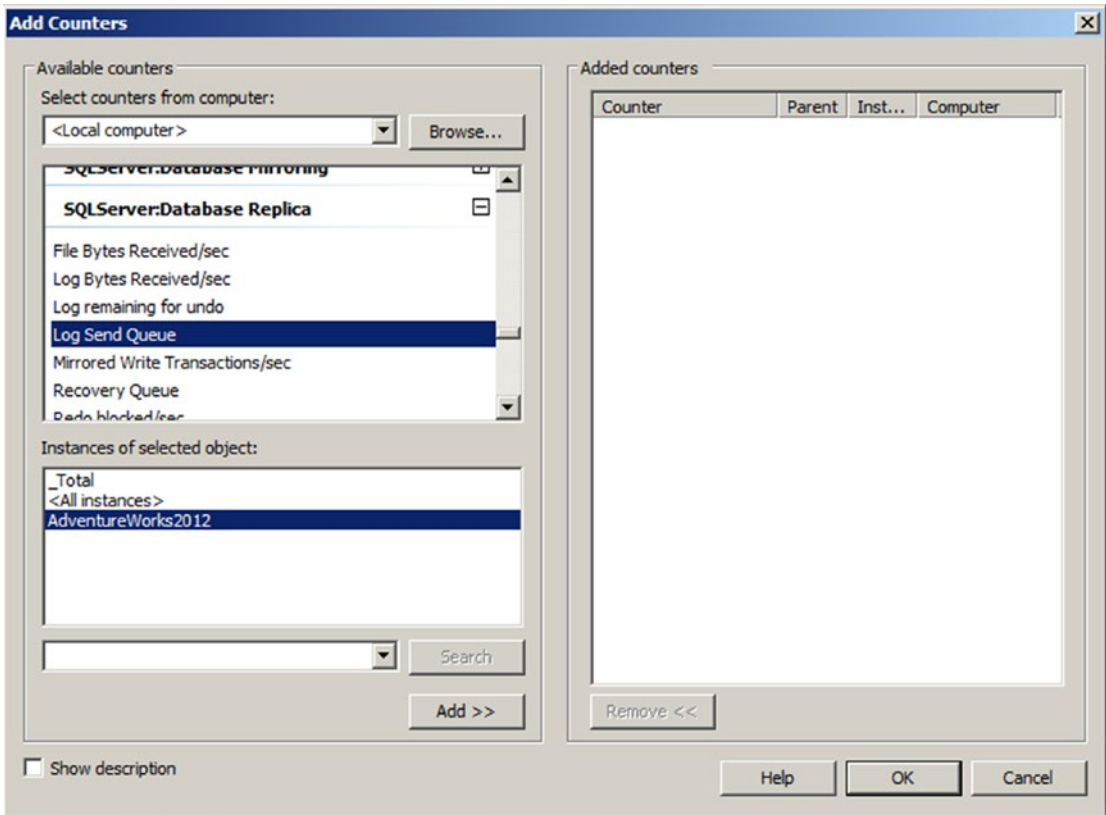
Figure 10-14. Perfmon counters related to AlwaysOn
