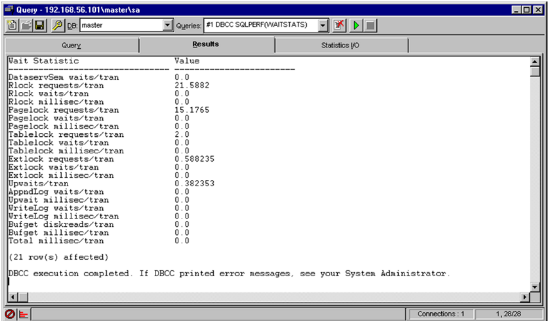
Figure 1-1. SQL Server wait statistics in SQL Server 6.5
