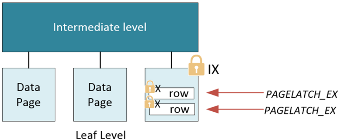
Figure 9-10. Leaf page of clustered index with locks in place
