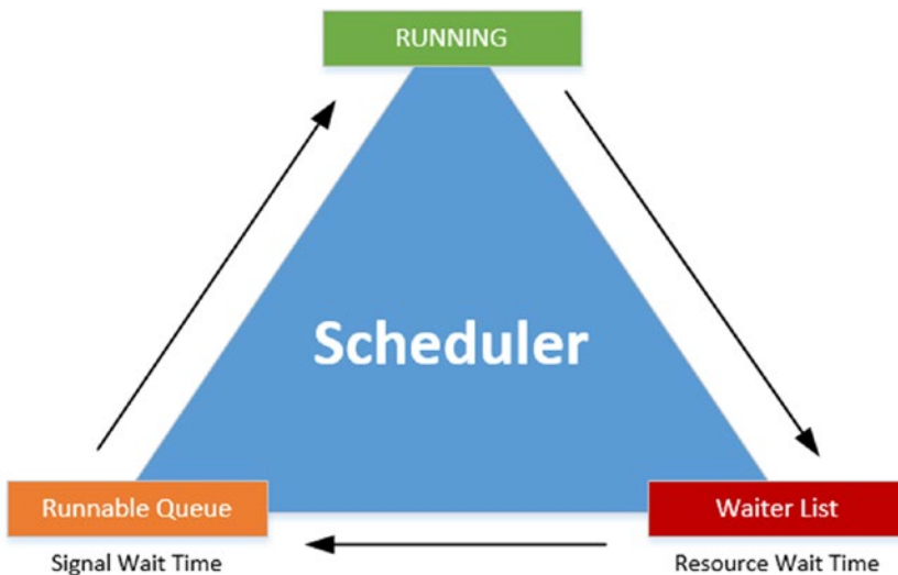
Figure 5-9. Scheduler and its phases and queues
