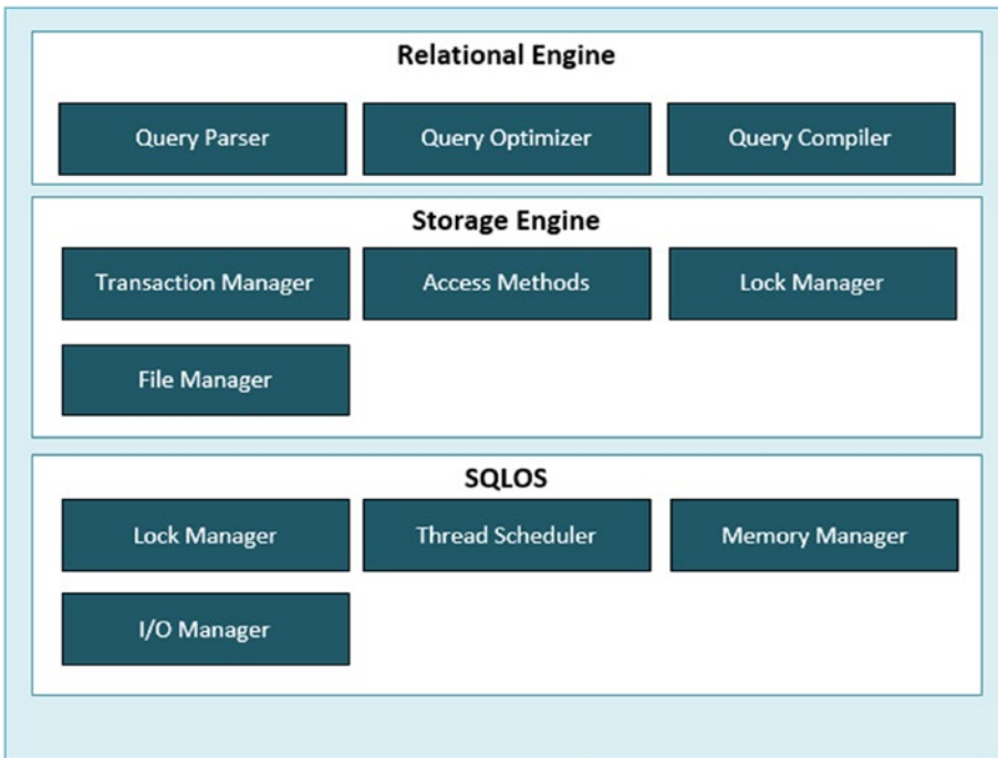
Figure 1-4. SQL Server 2005 architecture
