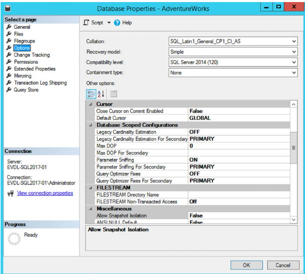
Figure 5-3. Database scoped parallelism configuration
