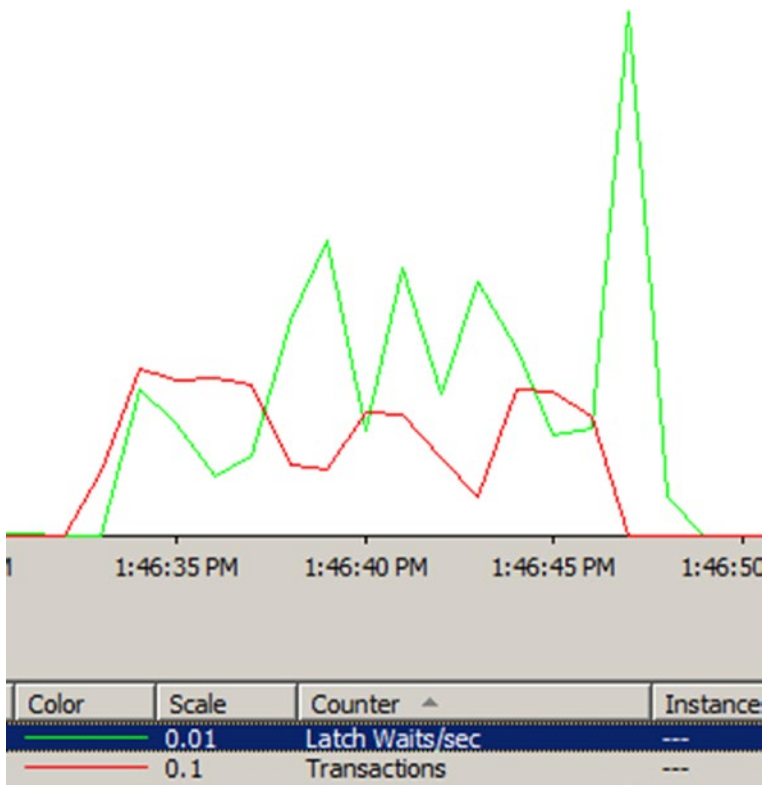
Figure 9-7. Latch Waits/sec and Transaction Perfmon graph after adding more TempDB files
