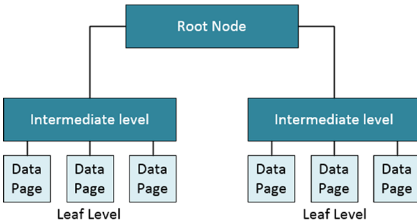
Figure 9-20. B-tree index structure
