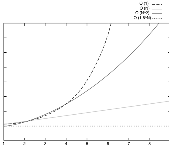
Figure 11.1 Comparing complexities.
