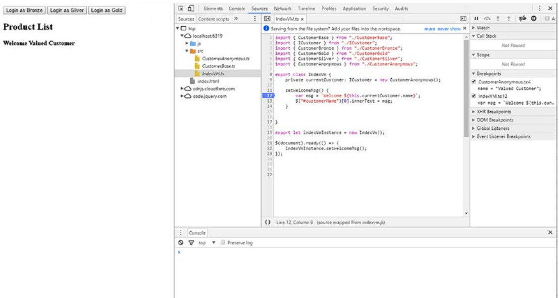
Figure 7-15. Breakpoint set
