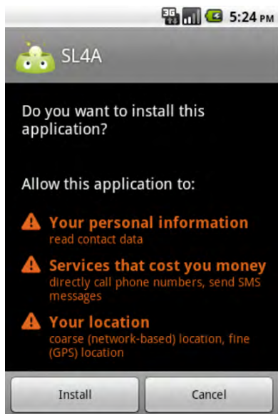
Figure 2-3. Installing SL4A
