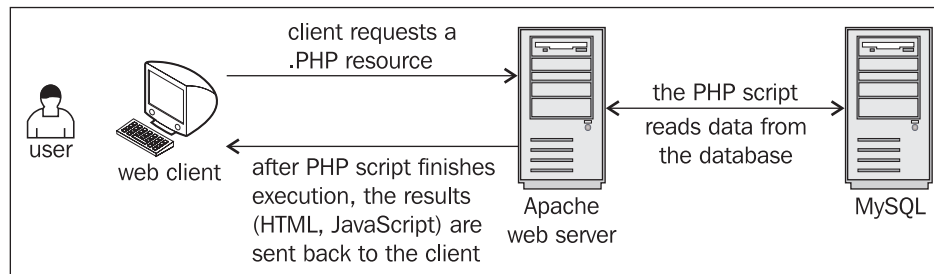
Figure 3.19: User Connecting to MySQL through Layers of Functionality
