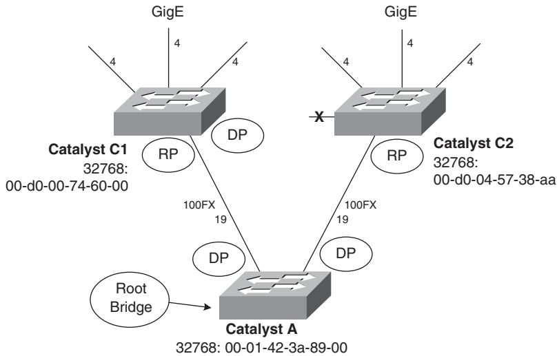
Figure 7-2 Network Diagram Demonstrating Poor STP Root Placement
