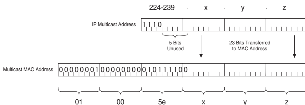
Figure 9-1 Multicast Address Translation
