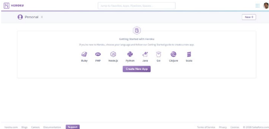
Figure 4-11. Heroku dashboard
