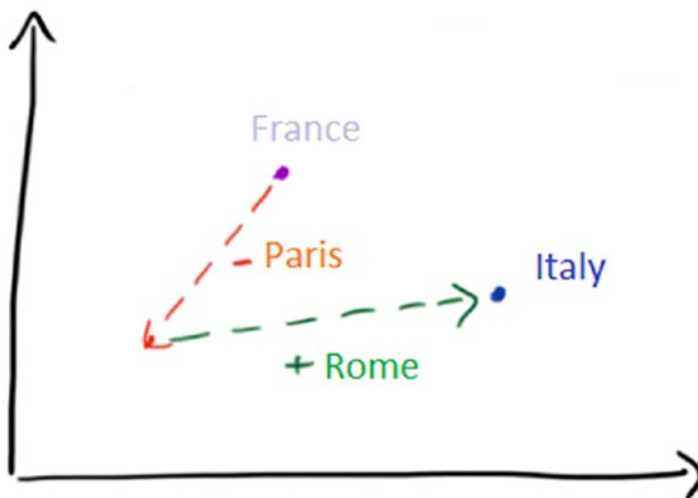
Figure 2-4. Comparing vectors
