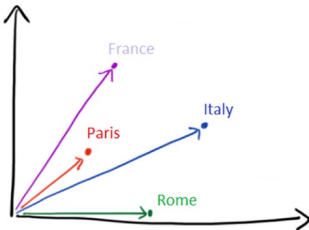
Figure 2-3. Our vectors
