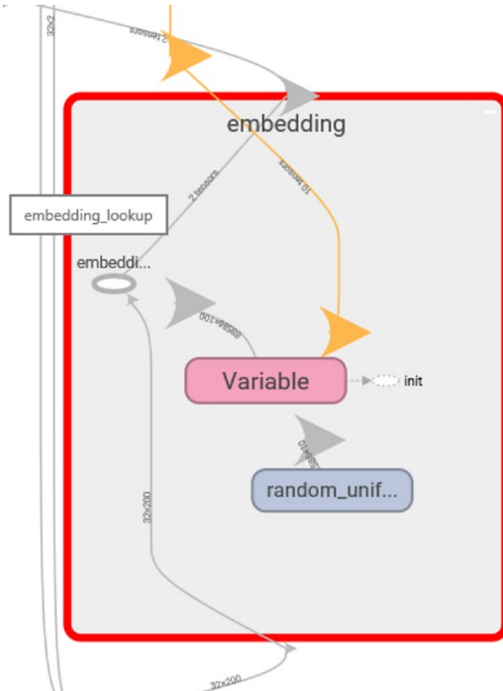
Figure 5-9. TensorBoard graph for the embedding segment
