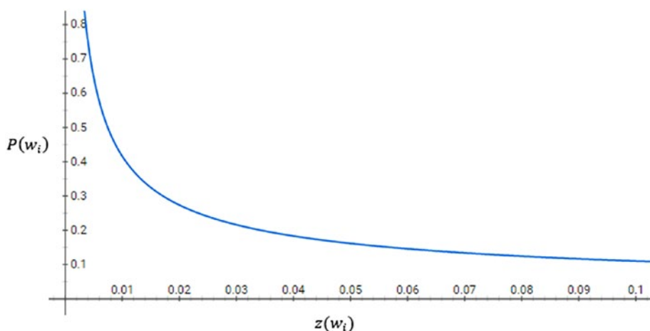
Figure 2-12. Distribution of the Survival function, P(x) = \{(\text{sqrt}(x/0.001) + 1) * (0.001/x)\} for a constant value of 0.001 for sampling rate (Credits : http://www.mccormickml.com )
