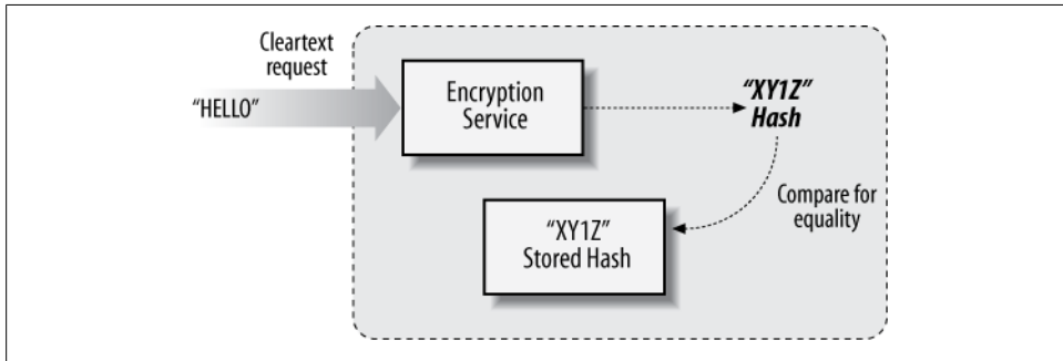
Figure 5-3. Comparing input with a hash of the expected result
