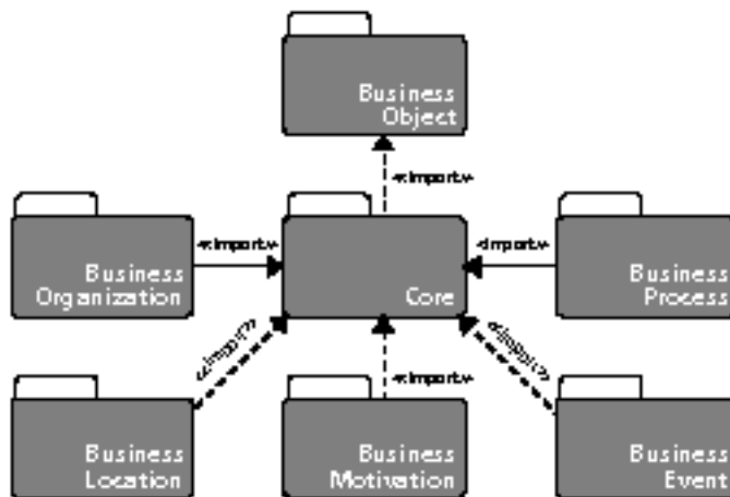
Fig. 2 The BML package structure
