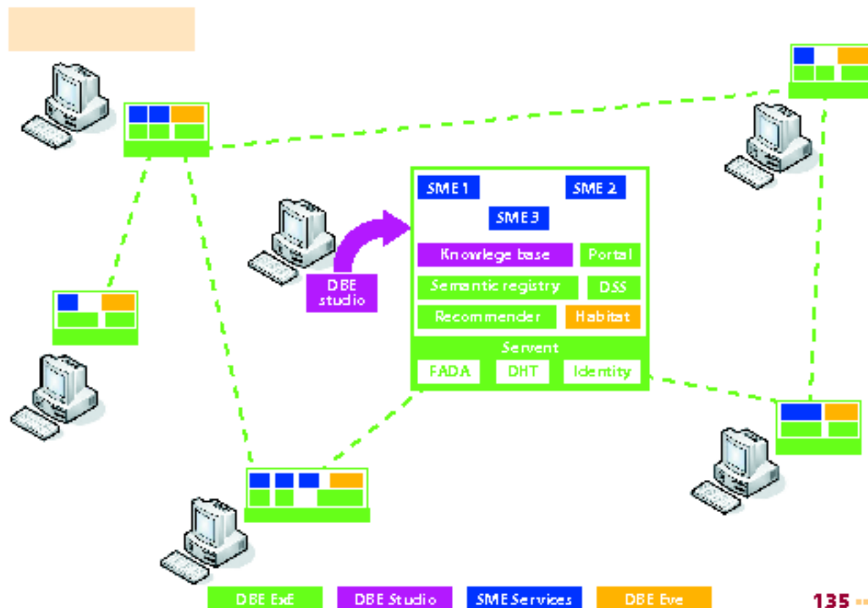
Fig. 1 Distributed Infrastructural Services of the DEE
