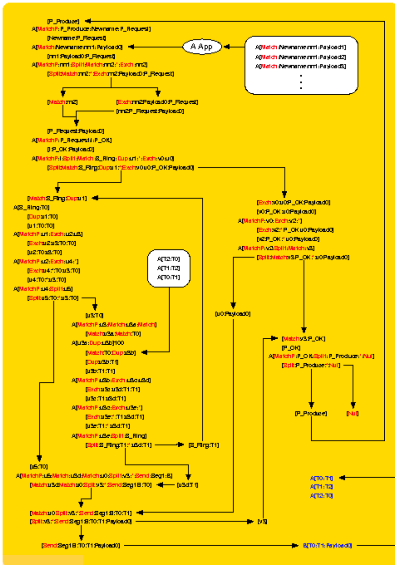
Fig. 1.3 Regular example showing the explicit algorithm (regular text) along with the implicit initial target multiset (bold)
