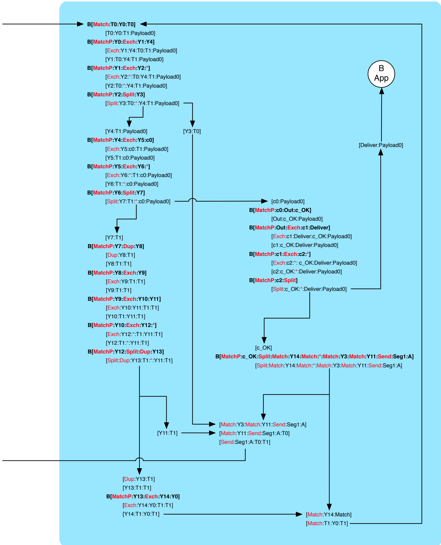
Credit-based flow control with reordering (C. Tschudin & L. Yamamoto, UBASEL; visualisation by P. Dini, LSE)
