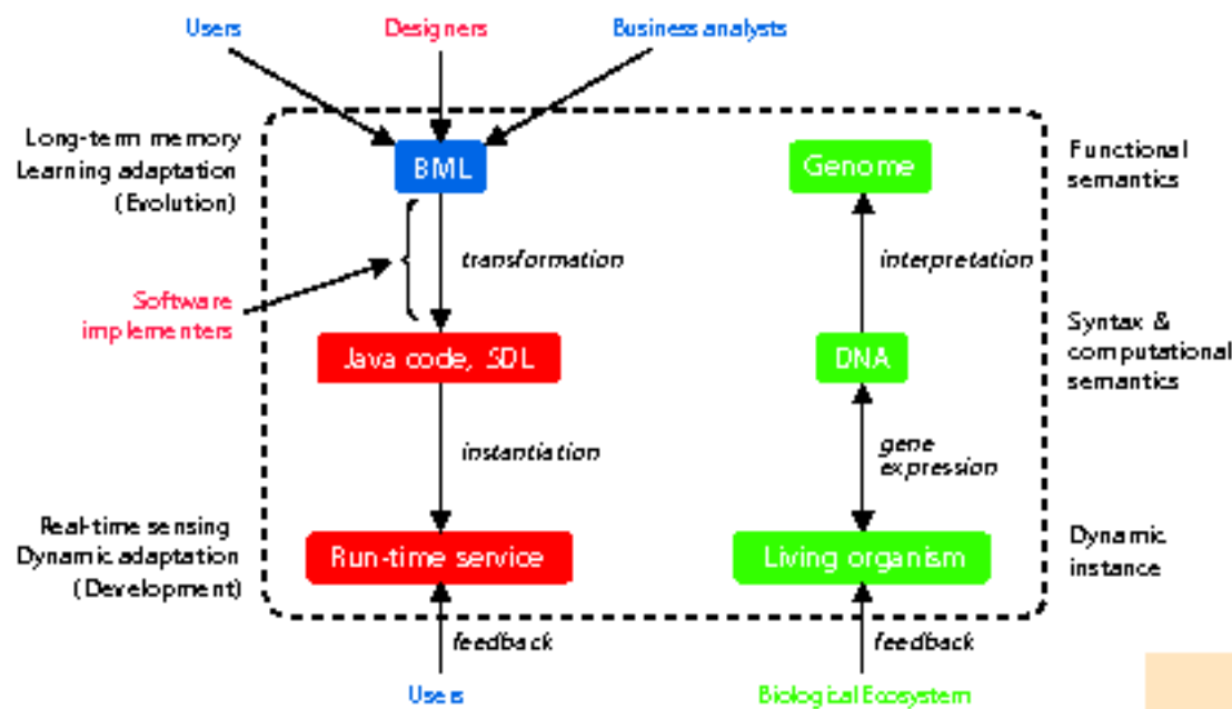
Fig. 16 Higher level analogy between software engineering and gene expression workflows
