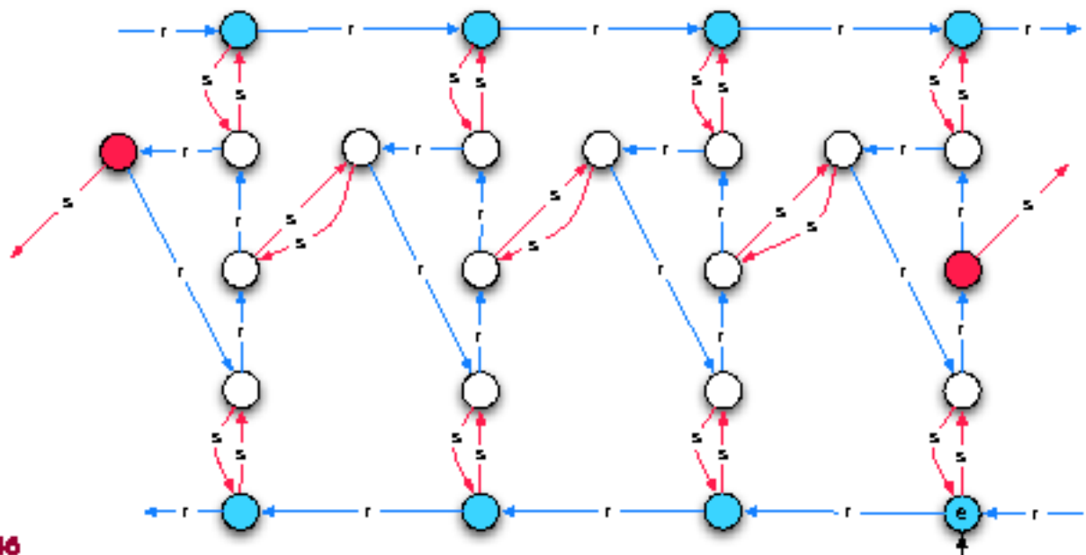
Fig. 1.13 D_6 isomorphic to the symmetries of the cube
