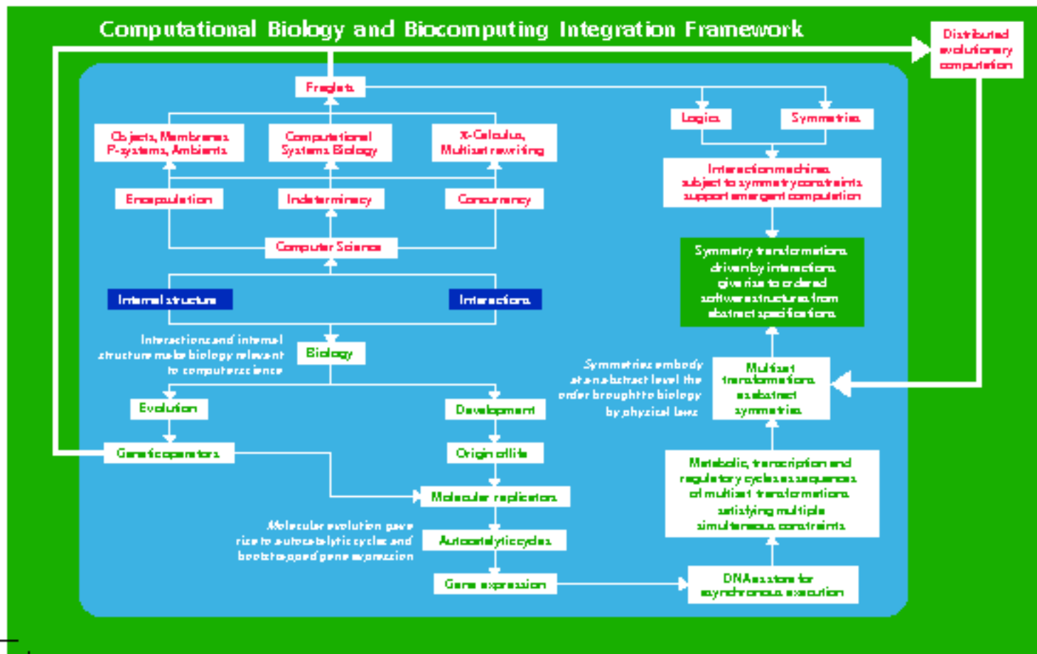
Fig. 1.6 Towards common mathematical framework for biology and computer science
