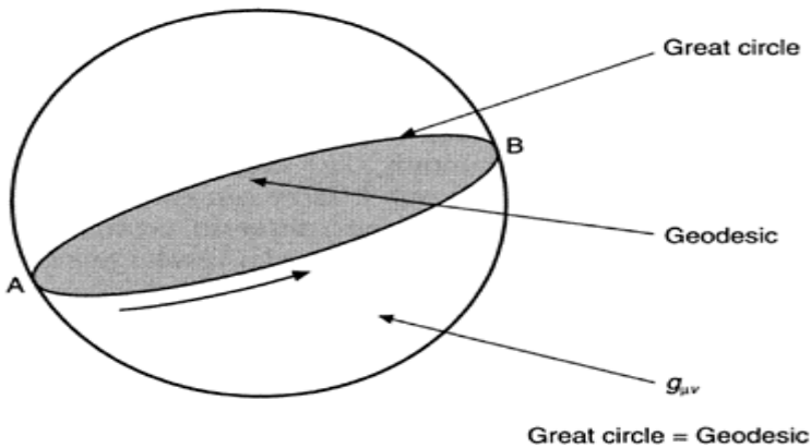
Figure 6.2 Geodesic on the simple sphere geometry (designed by Sang Wook Yi).
