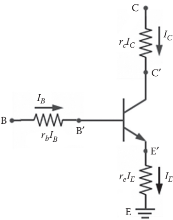
FIGURE 11.14 The parasitic series resistances on a typical npn -BJT device causing ohmic voltage drop at the respective neutral regions of the device.
