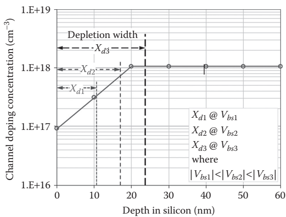
FIGURE 8.8 A piecewise graded-retrograde MOSFET channel doping profile from the silicon/SiO 2 interface at depth x = 0 into the substrate; here X_{d1} , X_{d2} , and X_{d3} are the depletion width due to the applied body bias V_{bs1} , V_{bs2} , and V_{bs3} , respectively, causing V_{th}(V_{bs}) variability due to RDD along the depth of the channel. (Data from S.K. Saha, IEEE Access , 2, 104–115, 2014.)
