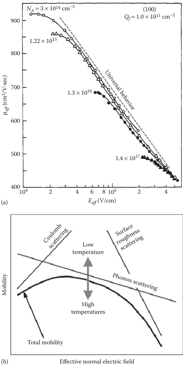
FIGURE 5.9 Low field mobility of inversion carriers in MOSFETs: (a) universal mobility behavior of inversion layer electrons in nMOSFET devices (Data from S.C. Sun and J.D. Plummer, IEEE Trans. Electron Dev. , 27, 1497–1508, 1980.) and (b) physical mechanisms showing the dependence of the inversion layer mobility on the effective vertical electric field.
