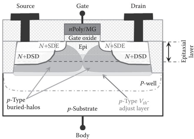
FIGURE 8.10 A variability-tolerant buried-halo MOSFET (BH-MOSFET) device structure; multiple halo implants are buried under the epitaxial layer to obtain undoped or lightly doped channel region.
