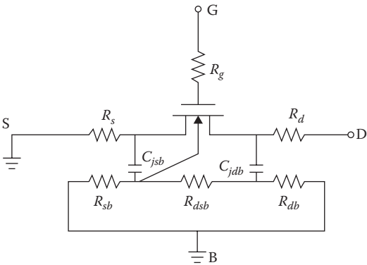
FIGURE 7.7 A subcircuit with parasitic elements added to an intrinsic MOSFET model for RF analysis. (Data from Y. Cheng et al., Proceedings of the ICSICT , 416–419, 1998.)
