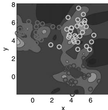
FIGURE 2.7: (SEE COLOR INSERT) Contours and the scores of six features. Among these features, F_1 and F_2 are relevant, and F_3, F_4, F_5 , and F_6 are irrelevant.
