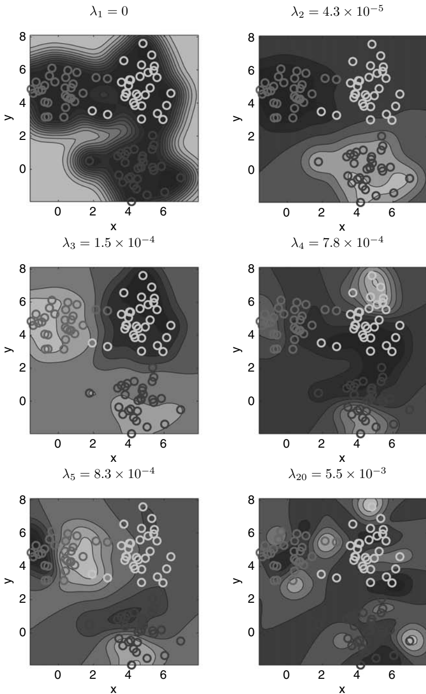
FIGURE 2.3: (SEE COLOR INSERT) Contours of the eigenvectors \xi_1, \xi_2, \xi_3, \xi_4, \xi_5, and \xi_{20} of \mathbf{L} .
