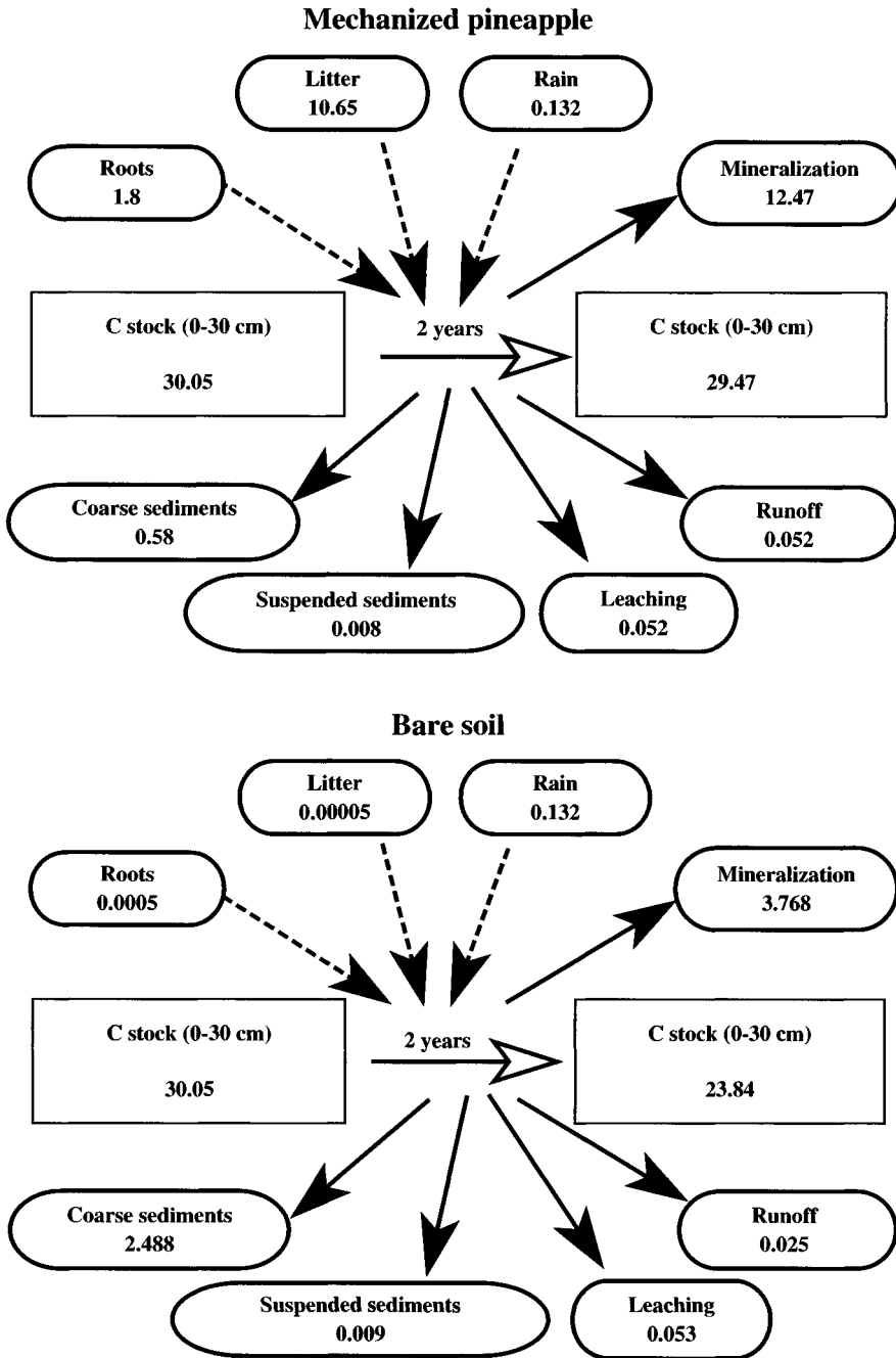
Figure 7.2 C budget in intensive-till pineapple and bare soil treatments (10% slope) showing C stock changes in 2 years (equivalent mass basis) (in Mg C ha -1 ), C inputs (litter, root, and rain) and C outputs (erosion, leaching, and mineralization) (in Mg C ha -1 2 yr -1 ).
