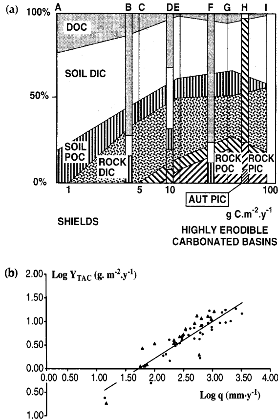
Figure 15.24 Exportation of total carbon by rivers. (a) Decomposition of carbon species exportation in a gradient of total carbon (TC) exportation \text{g C m}^{-2} \text{ yr}^{-1} . A = Gambia, B = Zaire, C = Mississippi, D = Solimoes, E = Chiang Jiang, F = Negro, G = Brahmaputra, H = Huang He, I = Dranse. (Data from Meybeck, M. 1993a. C, N, P, and S in rivers: From sources to global inputs, in R. Wollast, F. T. Mackenzie, and L. Chou, eds., Interaction of C, N, P and S Biogeochemical Cycles and Global Change . Springer-Verlag, pp. 163–193.) (b) Yield of riverine total atmospheric carbon ( \text{g C m}^{-2} \text{ yr}^{-1} ) vs. runoff ( \text{mm yr}^{-1} ) for major rivers. (Data from Meybeck and Ragu 1996, triangles: highly carbonated basins, log-log scale.)
