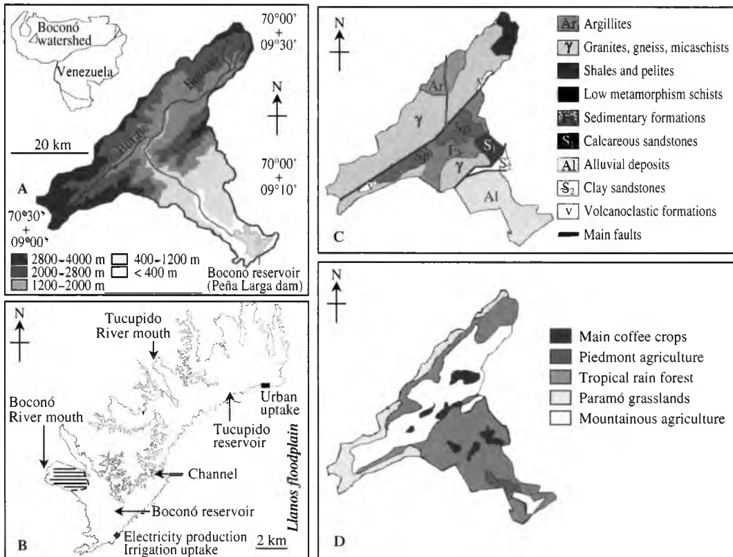
Figure 20.2 Location of the Rio Boconó watershed in Venezuela with main physiographic characteristics (a) altitudes, (b) physiographic map of the Peña Larga water dam at the outlet of the Rio Boconó watershed with open and black circles refer to sampling locations in September 1999. (Modified from Bellanger, B., S. Huon, P. Steinmann, F. Chabaux, F. Velasquez, V. Vallès, K. Arn, N. Clauer, and A. Mariotti. 2004a. Applied Geochemistry , 19, 1295–1314. With permission.) (c) Simplified lithological map, and (d) simplified vegetation cover. (Modified from Bellanger, B., S. Huon, F. Velasquez, V. Vallès, C. Girardin, and A. Mariotti. 2004b. Catena , 58, 125–150. With permission.)
