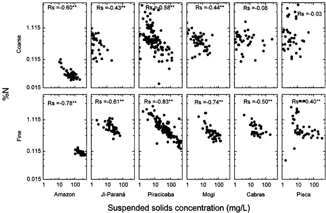
Figure 16.4 Plot of %N vs. suspended solids concentrations for the coarse and fine size fractions in the Amazon, Ji-Paraná, Piracicaba, Mogi, Cabras, and Pisca river watersheds.
