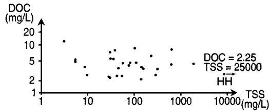
Figure 15.8 Dissolved organic carbon (DOC) variations vs. total suspended solids (annual averages). Note the specific position of the Huang He (HH).
