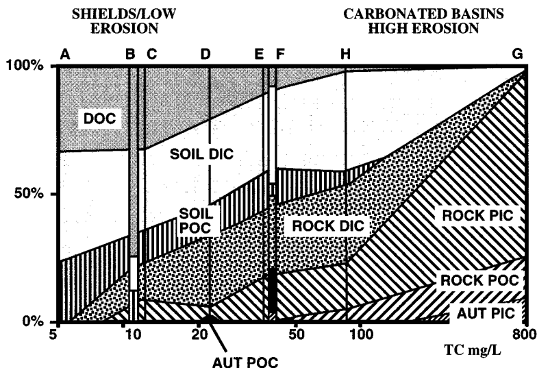
Figure 15.1 Origins of carbon species in selected rivers with increasing total carbon (TC) concentrations (annual averages). Soil-derived carbon: DOC, soil DIC, soil POC. Rock-derived carbon: rock DIC, rock PIC, rock POC. River-derived carbon: autochthonous (algal) POC, autochthonous PIC (in black). A = Gambia (West Africa), B = Rio Negro (Brazil), C = Solimoes (Brazil), D = Loire (winter average), E = Mackenzie, F = Loire (summer average), G = Huang He, H = Dranse (French Alps). (Data from Meybeck, M. 1993a. C, N, P, and S in rivers: From sources to global inputs, in R. Wollast, F. T. Mackenzie, and L. Chou, eds., Interaction of C, N, P, and S Biogeochemical Cycles and Global Change . Springer-Verlag, pp. 163–193.)
