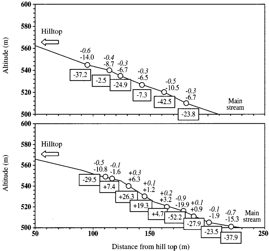
Figure 20.5 Distribution of soils along the two toposequences of the Houay Pano catchment (Laos). TOC changes (in gC m -2 yr -1 ) are included in rectangles. Soil redistribution rates (in kg m -2 yr -1 ) in italic and predicted TOC redistribution (in gC m -2 yr -1 ) are reported above the slope line.
