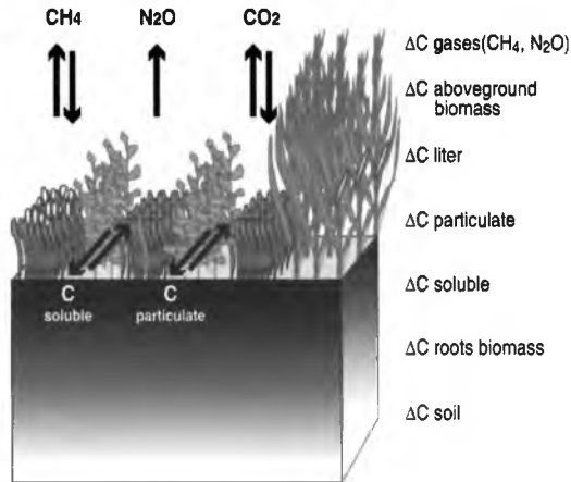
Figure 2.1 Fluxes (arrows) and changes ( \Delta ) that need to be accounted, at the plot level, for a complete comparison of the C and GWP balances for a given agroecosystem.
