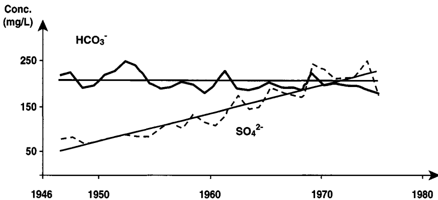
Figure 15.15 Bicarbonate sand sulfate trends in the Kura (Caucasus, 188,000 km 2 ). (From Nikanorov and Tsirkunov, 1984.)
