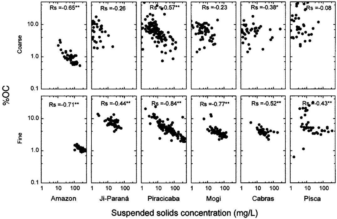
Figure 16.3 Plot of %OC vs. suspended solids concentrations for the coarse and fine size fractions in the Amazon, Ji-Paraná, Piracicaba, Mogi, Cabras, and Pisca river watersheds.
