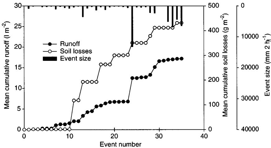
Figure 12.3 Mean cumulative runoff and soil losses at the 0.6-ha catchment outlet during the 2022 rainy season as a function of the rainfall event size.
