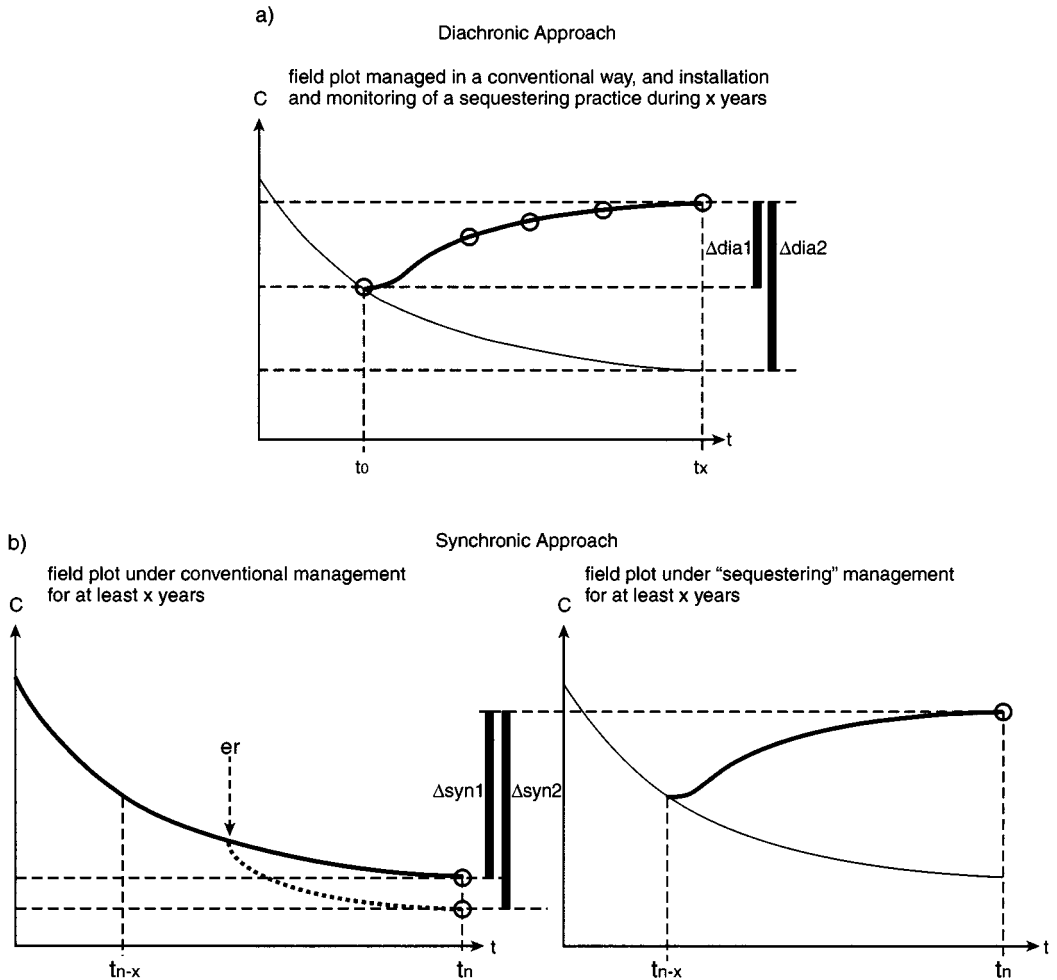
Figure 2.2 Comparison of the diachronic (a) and synchronic (b) approaches. Black circles correspond to C stocks determination; "er" stands for erosion.
