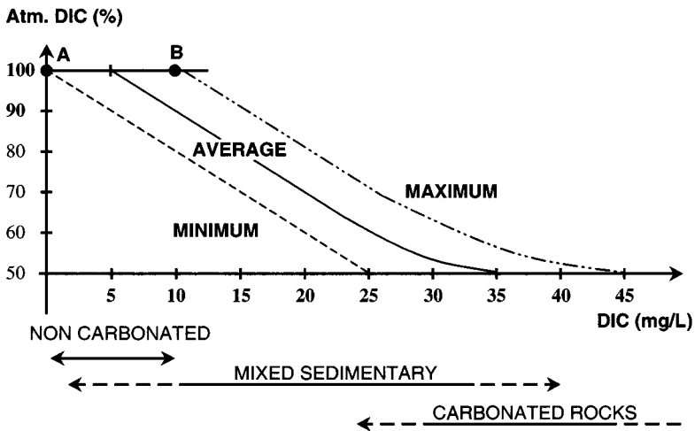
Figure 15.27 Model of DIC origins in river basins with variable proportions of carbonated rocks (% atmospheric DIC vs. total DIC as a function of average DIC level). Range of noncarbonated basins: A = Caroni, B = Reunion and Blue Nile.
