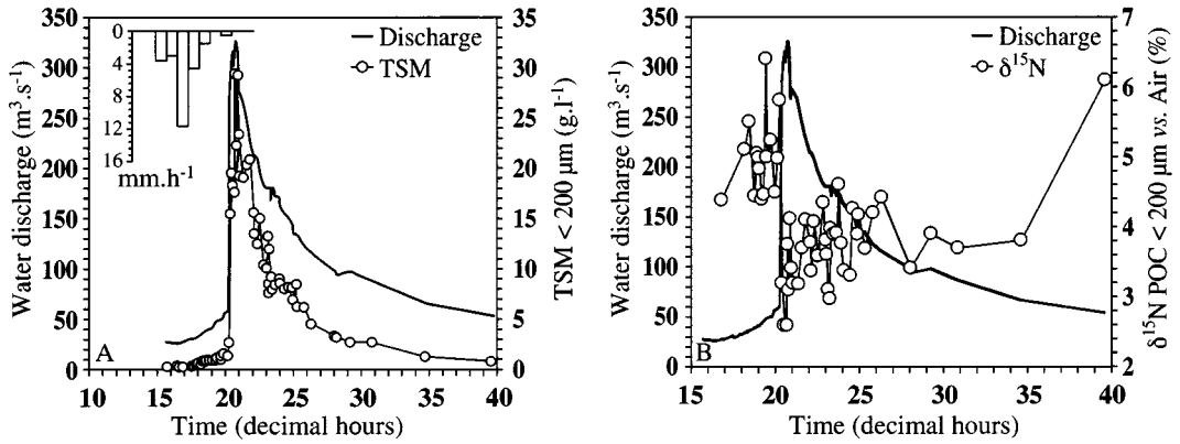
Figure 20.11 Plots of water discharge and (a) TSM delivery and (b) \delta^{15}\text{N} of suspended fine-size (< 200 \mu\text{m} ) fractions for the Rio Burate (Rio Boconó watershed, Venezuela) during the July 9 and 10, 1995 flood event. TSM = total suspended matter concentration.
