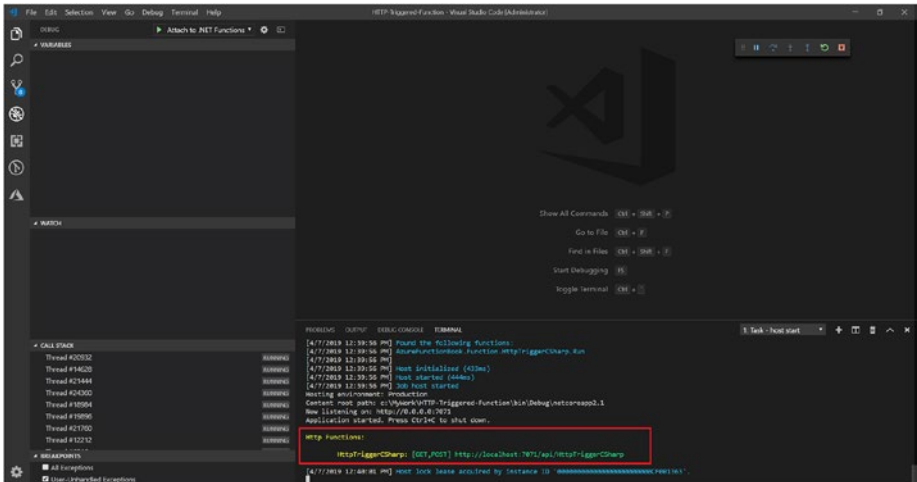
Figure 4-16. Local URL
