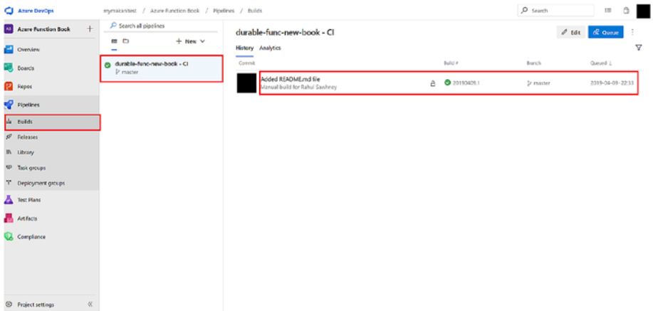
Figure 6-15. Build pipeline
