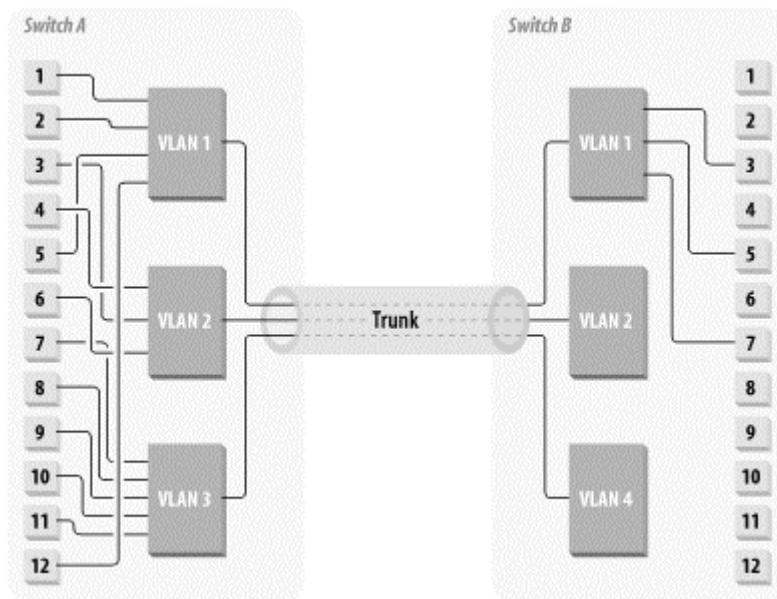
Figure 3-7. VLANs are shared through trunks
