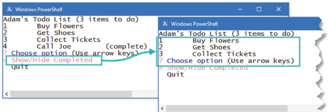
Figure 1-3. Toggling completed items
