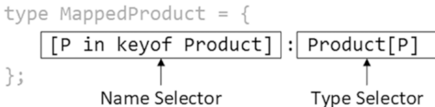
Figure 13-3. A mapped type
