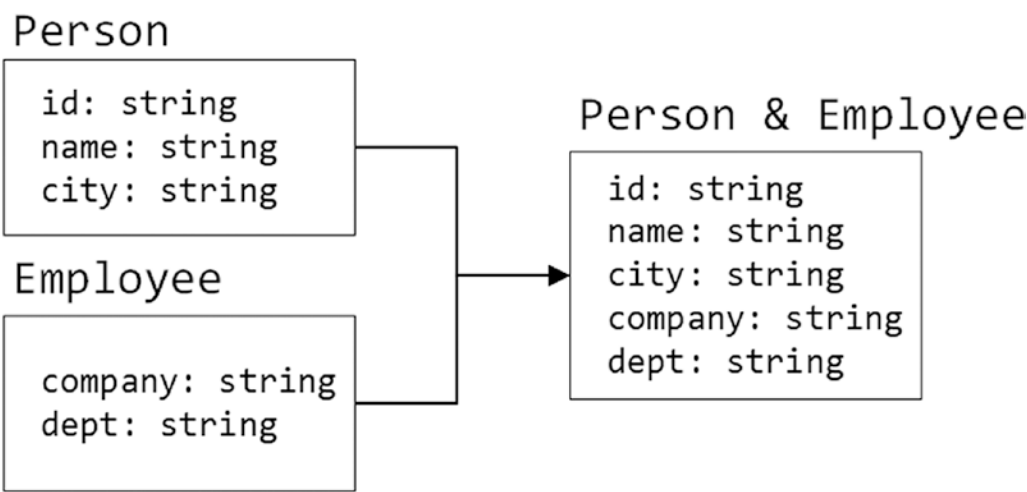
Figure 10-7. The effect of a type intersection
