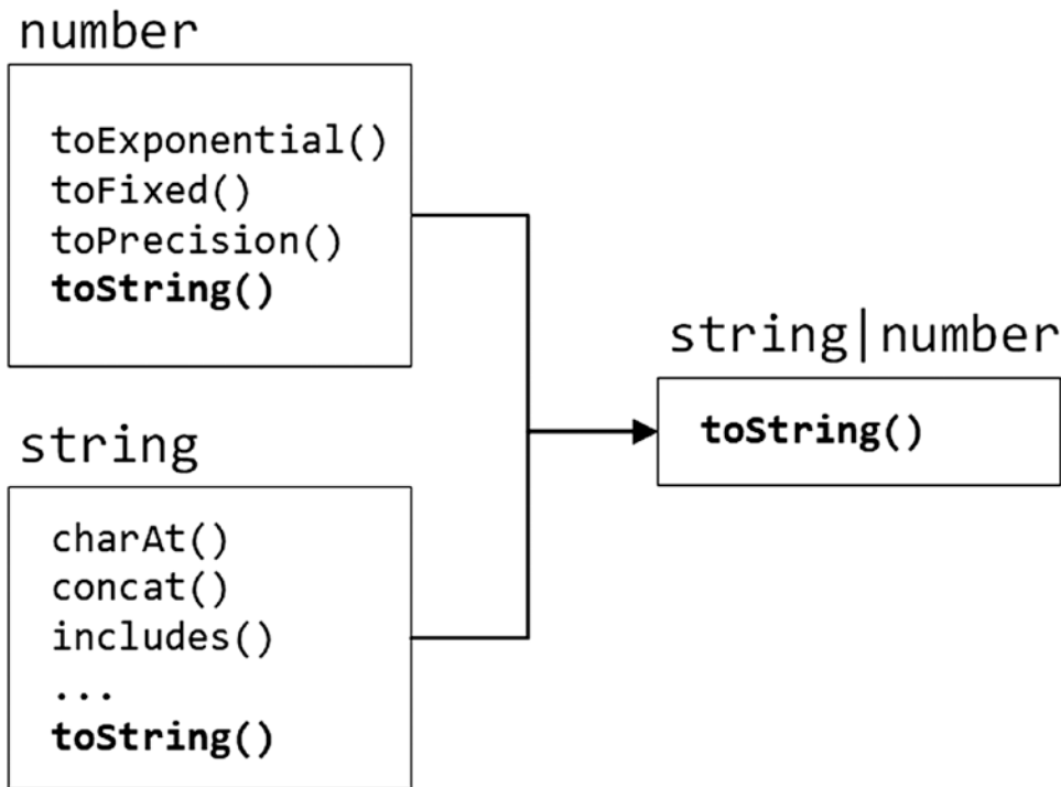
Figure 7-3 The effect of a type union
