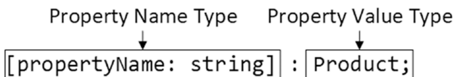
Figure 11-9. An index signature
