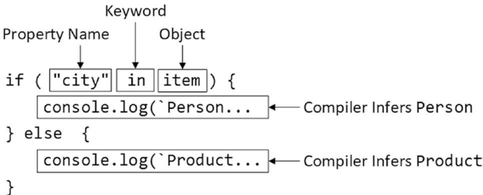
Figure 10-4. Using the in keyword
