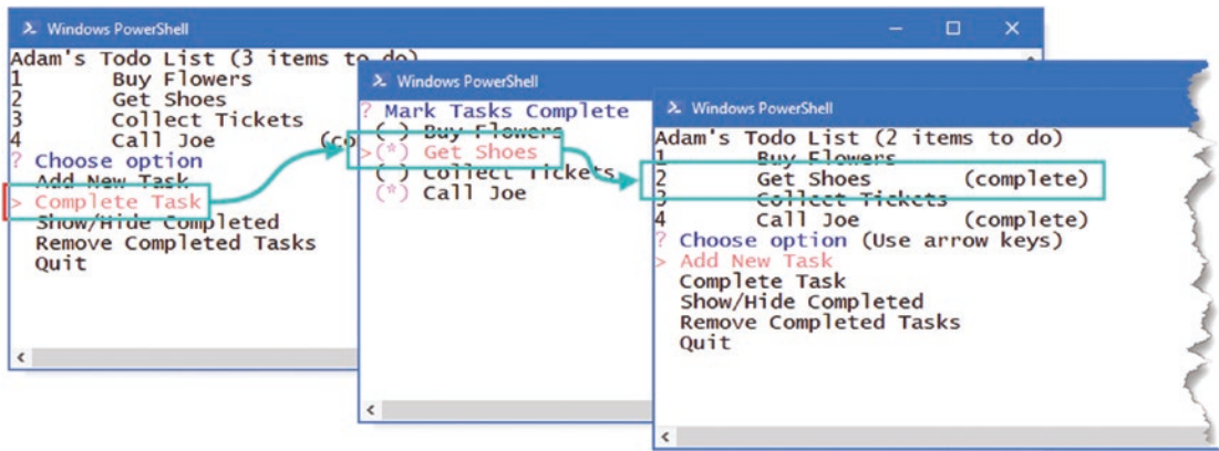
Figure 1-5. Completing items
