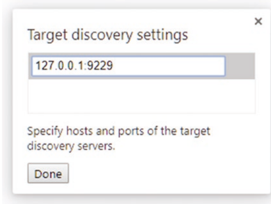
Figure 6-3. Configuring Chrome for remote Node.js debugging
