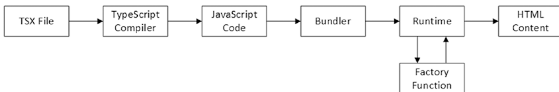
Figure 15-6. Transforming JSX
