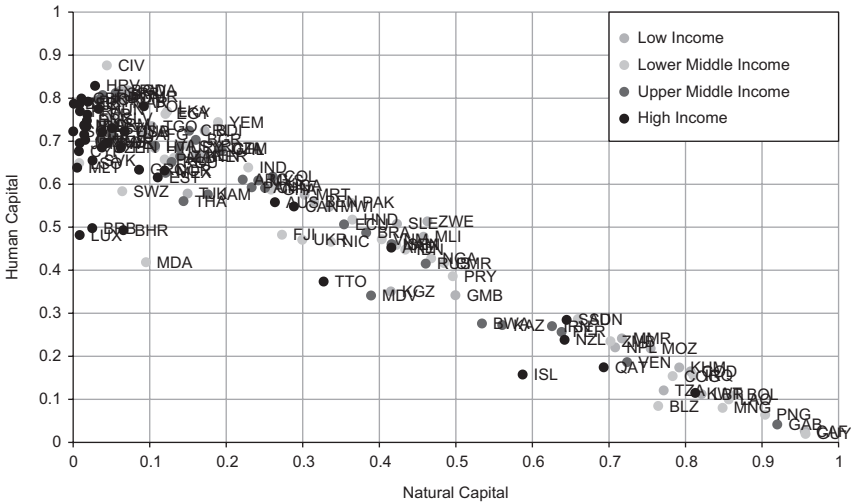
Figure 1.24c Percentage shares of human capital and natural capital in total wealth, average 1990–2014 (education approach)
