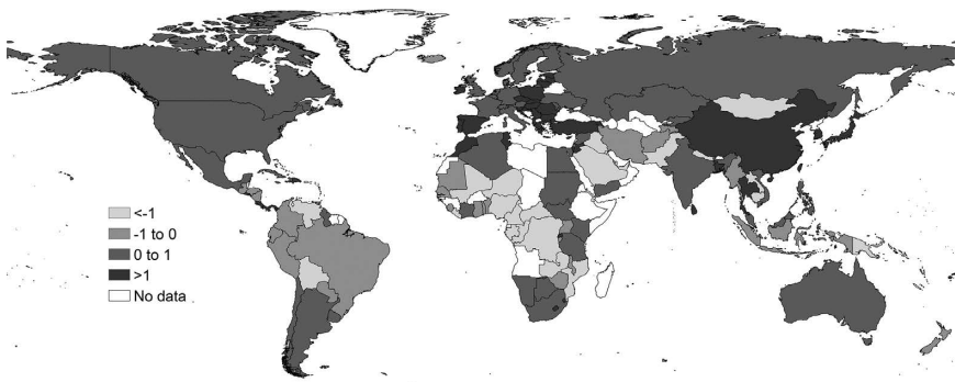
Figure 1.18b Growth in Inclusive Wealth Index per capita (unadjusted), using the education approach
