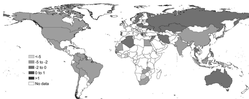
Figure 3.13 Average annual growth rate of minerals per capita from 1990–2014
