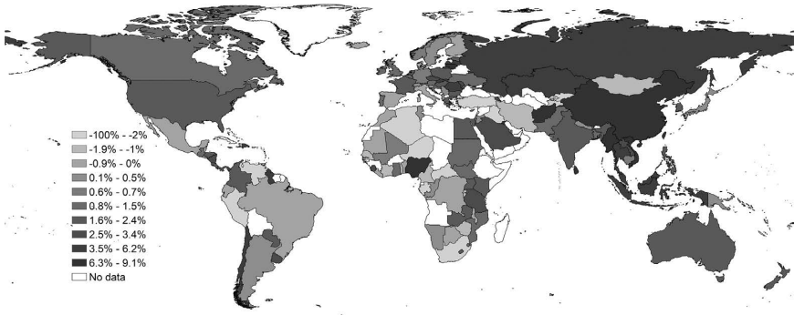
Figure 9.6 Growth of the PM2.5 damages per capita from 1990–2014 (percentage)
