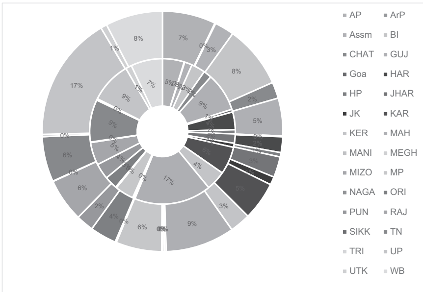
Figure 6.1 States share of GDP and population in 2011
