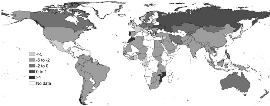
Figure 3.9 Average annual growth rate of non-renewables per capita from 1990–2014
