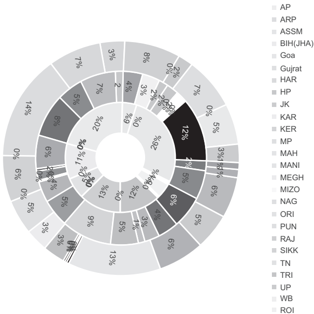
Figure 6.5 Share of forest, subsoil assets and human capital in Indian states Source: Based on author’s estimates.
