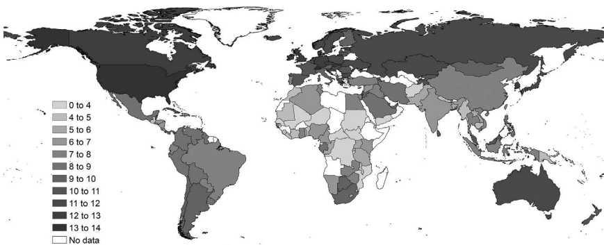
Figure 9.1 Average years of schooling from 1990 to 2014
