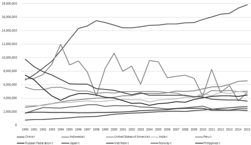
Figure 3.20 Top 10 countries in fishery capture production
