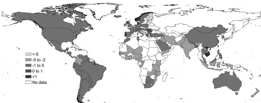
Figure 3.6 Average annual growth rate of pastureland per capita from 1990 to 2014
