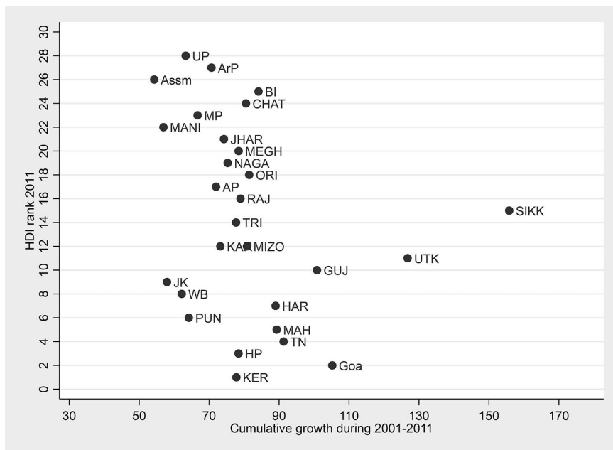
Figure 6.4 Decadal cumulative growth in GDP (2001–2011) vs. HDI 2011
