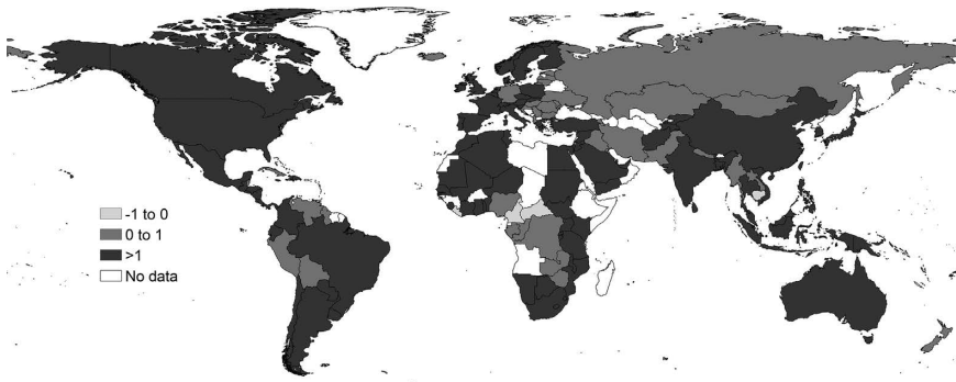
Figure 1.18a Growth in Inclusive Wealth Index (unadjusted), using the education approach
