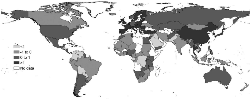
Figure 1.3b Annual average growth rate of Inclusive Wealth Index per capita
