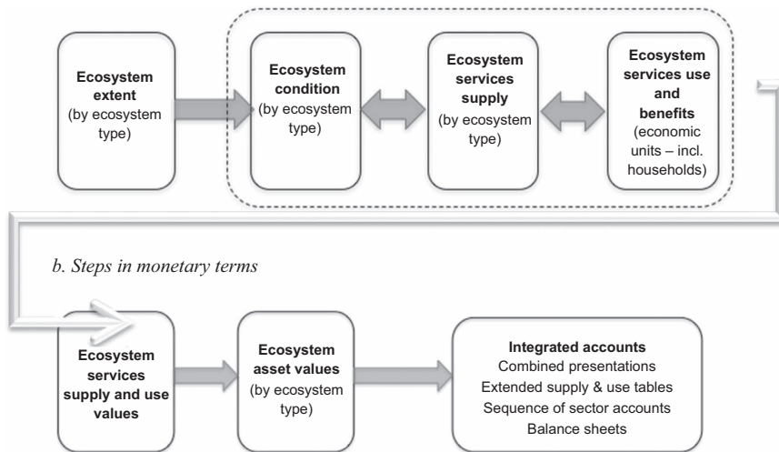
Figure 5.2 Broad steps in ecosystem accounting
