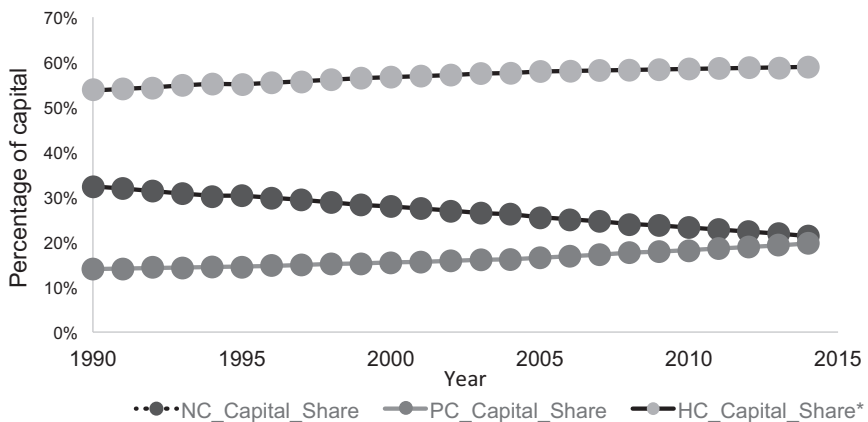
Figure 2.1 Global trend in human (HC), natural (NC) and physical (PC) capital shares
