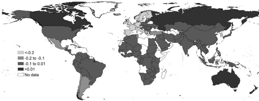
Figure 1.12c Average growth rate of carbon damage in 1990–2014
