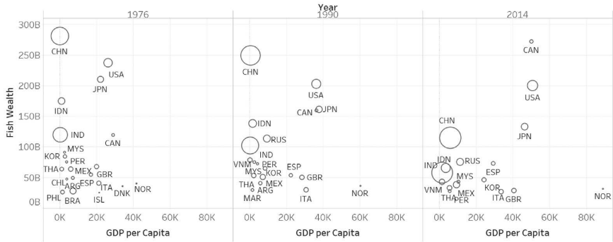
Figure 9.9 Comparison of fish stock capital for selected countries
