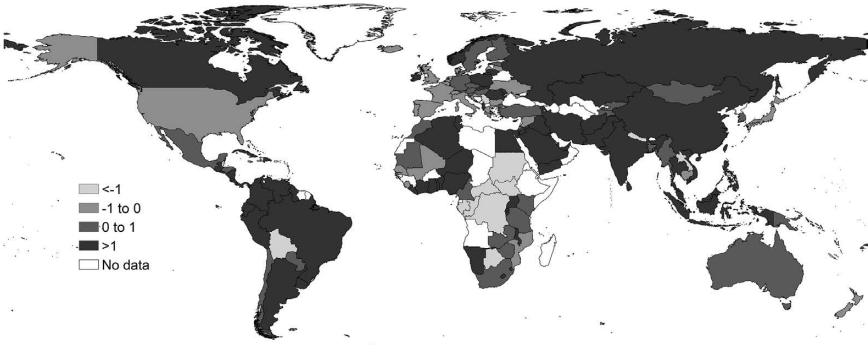
Figure 1.18c Growth in Inclusive Wealth Index per capita adjusted, using the education approach
