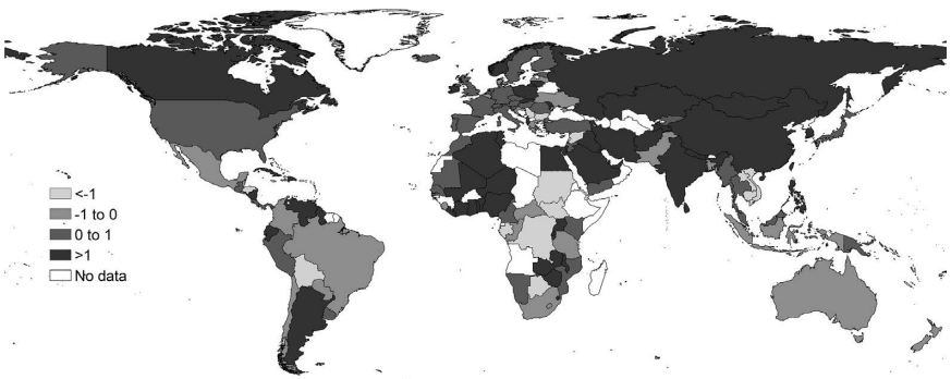
Figure 1.4b Growth in Inclusive Wealth Index per capita (adjusted)
