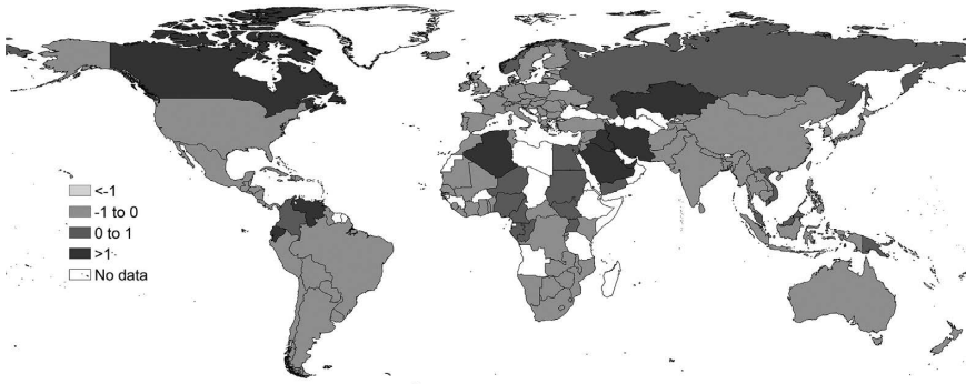
Figure 1.12a Average growth rate of oil capital gains in 1990–2014
