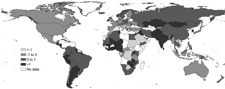
Figure 1.12b Average growth rate of Total Factor Productivity (TFP) in 1990–2014
