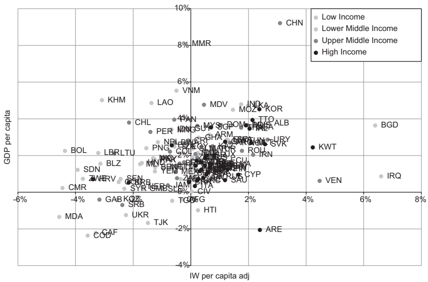
Figure 1.27b Growth rates in IW per capita adjusted (education approach) vs. GDP per capita
